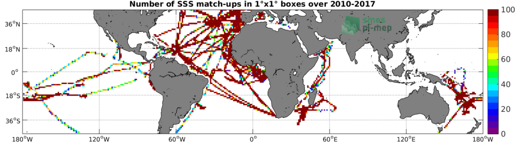
Figure 4: Number of SSS match-ups between TSG-GOSUD-Research-vessel SSS and the SMOS-L4-CATDS-CECOS-IFREMER-V2-WEEKLY-0.5DEG SSS product for the Mid-Low Latitudes 45N-45S Pi-MEP region over 1^\circ \times 1^\circ boxes and for the full satellite product period.
