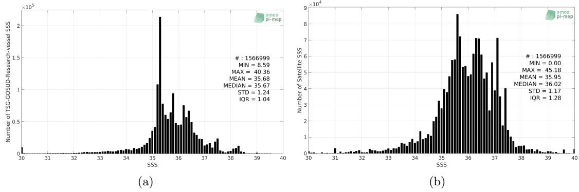
Figure 2: Histograms of SSS from TSG-GOSUD-Research-vessel (a) and SMOS-L4-CATDS-CECOS-IFREMER-V2-WEEKLY-0.5DEG (b) considering all match-up pairs per bins of 0.1 over the Mid-Low Latitudes 45N-45S Pi-MEP region and for the full satellite product period.
