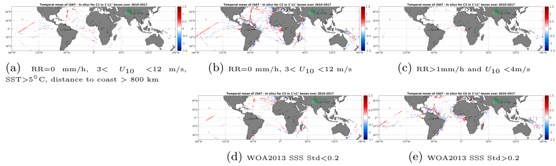
Figure 12: Temporal mean gridded over spatial boxes of size 1^\circ \times 1^\circ of \Delta SSS (SMOS-L4-CATDS-CECOS-IFREMER-V2-WEEKLY-0.5DEG - TSG-GOSUD-Research-vessel) for 5 different sub-datasets corresponding to: RR=0 mm/h, 3 < U_{10} < 12 m/s, SST > 5^\circ C , distance to coast > 800 km (a), RR=0 mm/h, 3 < U_{10} < 12 m/s (b), RR > 1 mm/h and U_{10} < 4 m/s (c), WOA2013 SSS Std < 0.2 (d), WOA2013 SSS Std > 0.2 (e).
