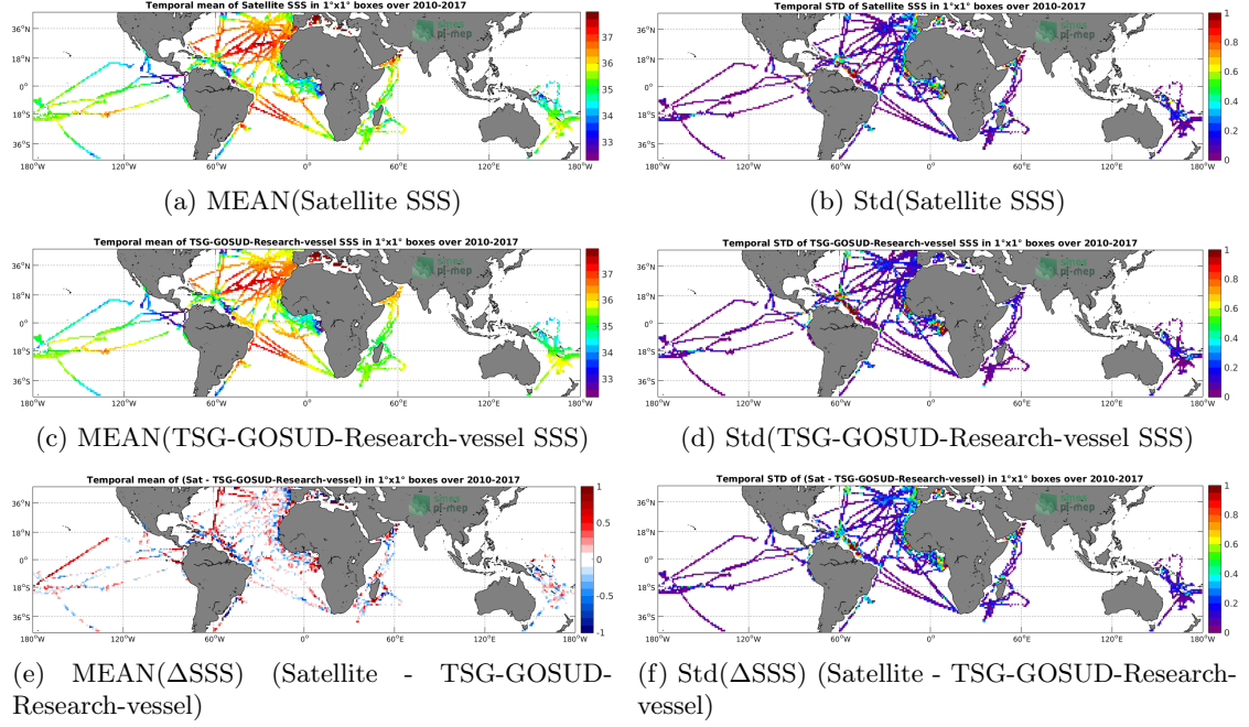
Figure 6: Temporal mean (left) and Std (right) of SSS from SMOS-L4-CATDS-CECOS-IFREMER-V2-WEEKLY-0.5DEG (top), TSG-GOSUD-Research-vessel (middle), and of \Delta SSS (Satellite - TSG-GOSUD-Research-vessel). Only match-up pairs are used to generate these maps.
