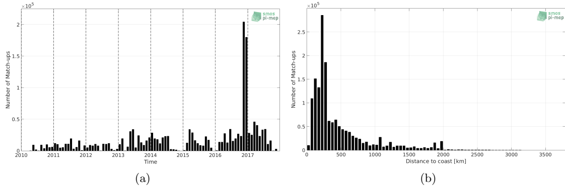
Figure 1: Number of match-ups between TSG-GOSUD-Research-vessel and SMOS-L4-CATDS-CECOS-IFREMER-V2-WEEKLY-0.5DEG SSS as a function of time (a) and as function of the distance to coast (b) over the Mid-Low Latitudes 45N-45S Pi-MEP region and for the full satellite product period.
