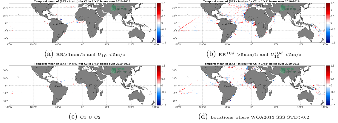
Figure 12: Temporal mean gridded over spatial boxes of size 1^\circ \times 1^\circ of \Delta SSS (SMOS-L4-CATDS-CECOS-IFREMER-V2-WEEKLY-0.5DEG - TSG-GOSUD-Research-vessel) for 4 different sub-datasets corresponding to: RR > 1mm/h and U_{10} < 5\text{m/s} (a), RR^{10d} > 5\text{mm/h} and U_{10}^{10d} < 5\text{m/s} (b), C1 U C2 (c), Locations where WOA2013 SSS STD > 0.2 (d).
