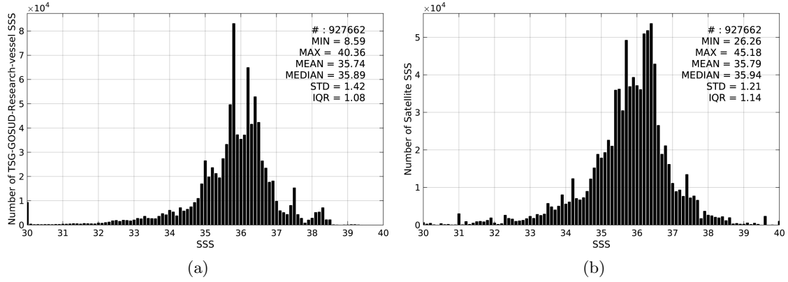
Figure 2: Histograms of SSS from TSG-GOSUD-Research-vessel (a) and SMOS-L4-CATDS-CECOS-IFREMER-V2-WEEKLY-0.5DEG (b) considering all match-up pairs per bins of 0.1 over the Mid-Low Latitudes 45N-45S Pi-MEP region and for the full satellite product period.
