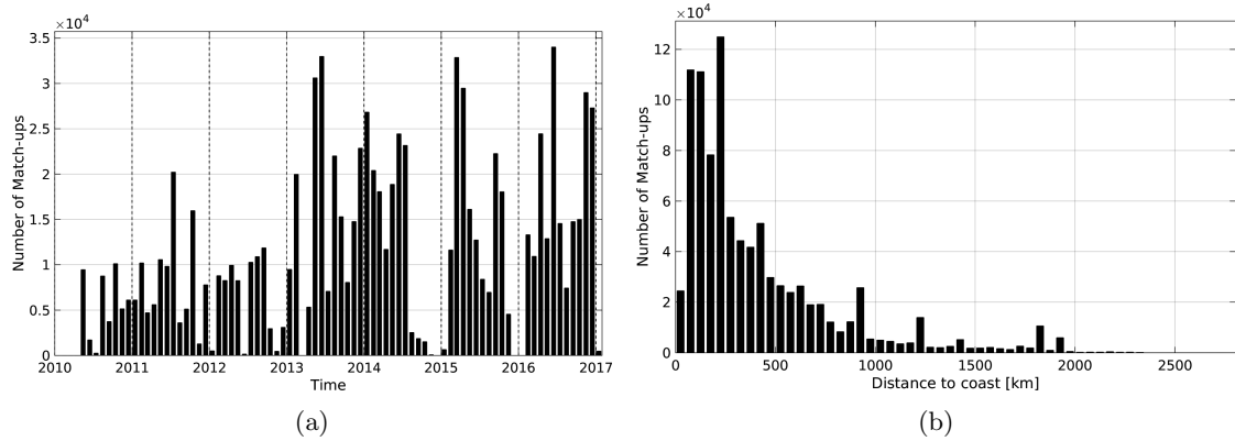
Figure 1: Number of match-ups between TSG-GOSUD-Research-vessel and SMOS-L4-CATDS-CECOS-IFREMER-V2-WEEKLY-0.5DEG SSS as a function of time (a) and as function of the distance to coast (b) over the Mid-Low Latitudes 45N-45S Pi-MEP region and for the full satellite product period.
