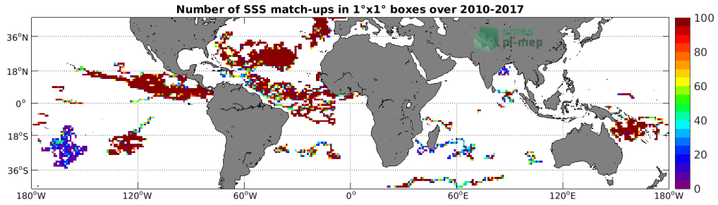
Figure 3: Number of SSS match-ups between Surface drifters SSS and the SMOS L4 v2 Weekly (CATDS-CECOS-IFREMER) SSS product for the Mid-Low Latitudes 45N-45S Pi-MEP region over 1°x1° boxes and for the full satellite product period.
