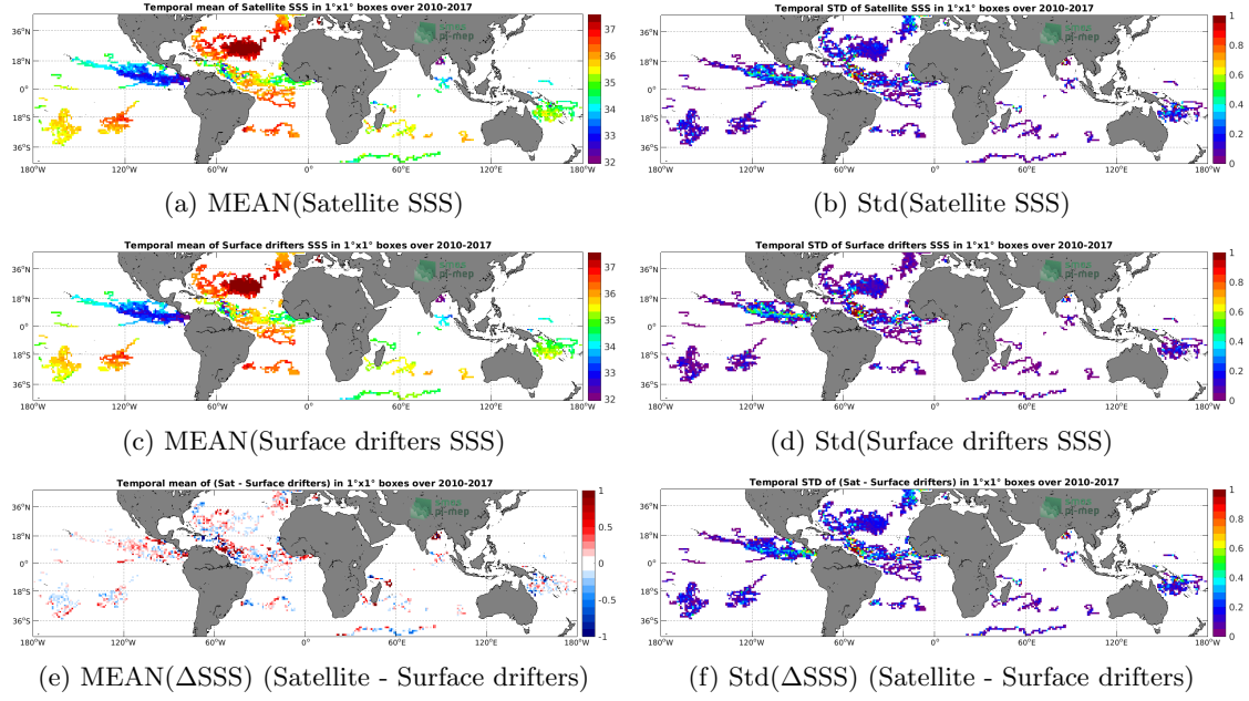
Figure 5: Temporal mean (left) and Std (right) of SSS from SMOS L4 v2 Weekly (CATDS-CECOS-IFREMER) (top), Surface drifters (middle), and of \Delta SSS (Satellite - Surface drifters). Only match-up pairs are used to generate these maps.
