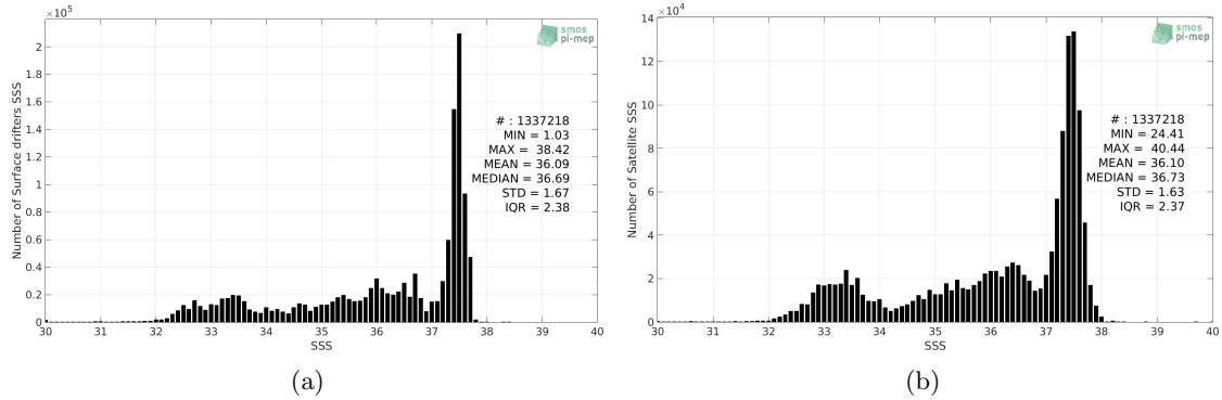
Figure 2: Histograms of SSS from Surface drifters (a) and SMOS-L4-CATDS-CECOS-IFREMER-V2-WEEKLY-0.5DEG (b) considering all match-up pairs per bins of 0.1 over the Mid-Low Latitudes 45N-45S Pi-MEP region and for the full satellite product period.
