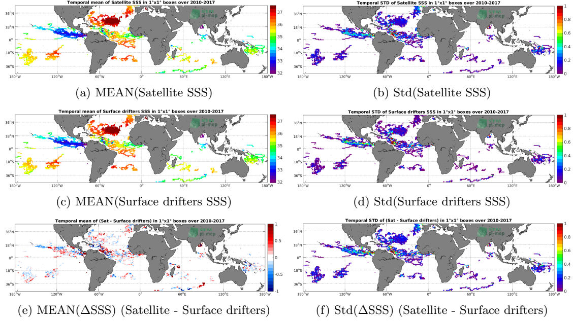
Figure 5: Temporal mean (left) and Std (right) of SSS from SMOS-L4-CATDS-CECOS-IFREMER-V2-WEEKLY-0.5DEG (top), Surface drifters (middle), and of \Delta SSS (Satellite - Surface drifters). Only match-up pairs are used to generate these maps.
