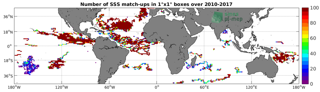
Figure 3: Number of SSS match-ups between Surface drifters SSS and the SMOS-L4-CATDS-CECOS-IFREMER-V2-WEEKLY-0.5DEG SSS product for the Mid-Low Latitudes 45N-45S Pi-MEP region over 1°x1° boxes and for the full satellite product period.
