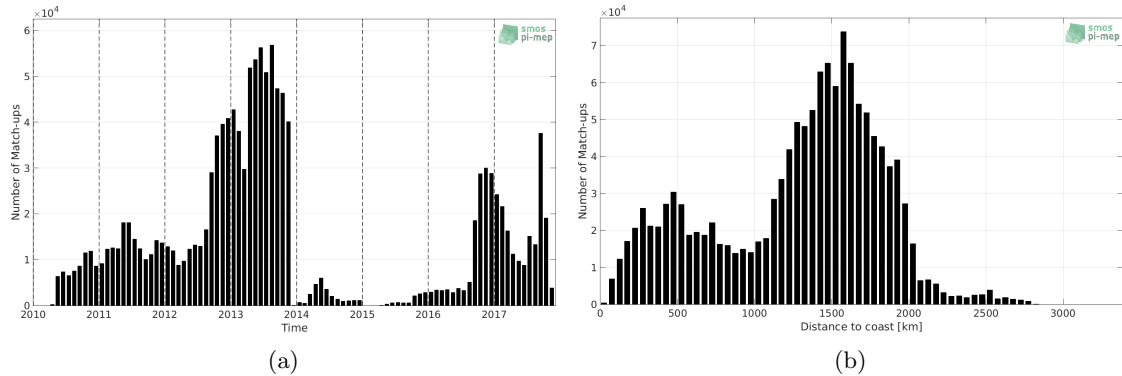
Figure 1: Number of match-ups between Surface drifters and SMOS-L4-CATDS-CECOS-IFREMER-V2-WEEKLY-0.5DEG SSS as a function of time (a) and as function of the distance to coast (b) over the Mid-Low Latitudes 45N-45S Pi-MEP region and for the full satellite product period.
