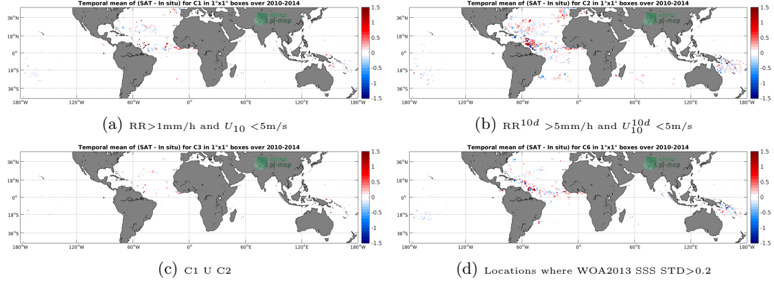
Figure 11: Temporal mean gridded over spatial boxes of size 1^\circ \times 1^\circ of \Delta SSS (SMOS-L4-CATDS-CECOS-IFREMER-V2-WEEKLY-0.5DEG - Surface drifters) for 4 different subdatasets corresponding to: RR > 1\text{mm/h} and U_{10} < 5\text{m/s} (a), RR^{10d} > 5\text{mm/h} and U_{10}^{10d} < 5\text{m/s} (b), C1 U C2 (c), Locations where WOA2013 SSS STD > 0.2 (d).
