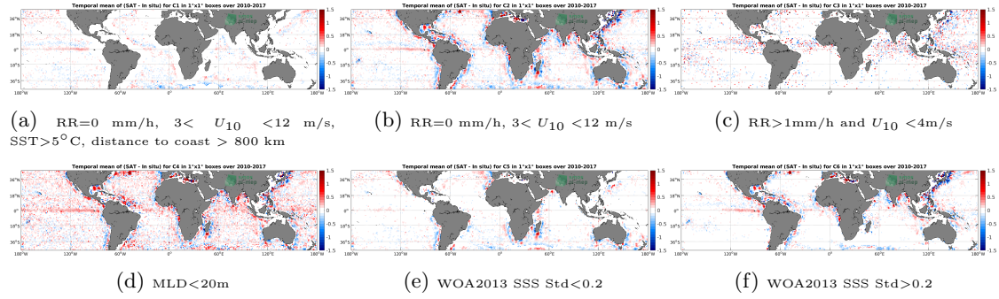
Figure 12: Temporal mean gridded over spatial boxes of size 1^\circ \times 1^\circ of \Delta SSS (SMOS L4 v2 Weekly (CATDS-CECOS-IFREMER) - Argo) for 6 different subdatasets corresponding to: RR=0 mm/h, 3 < U_{10} < 12 m/s, SST > 5^\circ C , distance to coast > 800 km (a), RR=0 mm/h, 3 < U_{10} < 12 m/s (b), RR > 1 mm/h and U_{10} < 4 m/s (c), MLD < 20 m (d), WOA2013 SSS Std < 0.2 (e), WOA2013 SSS Std > 0.2 (f).
