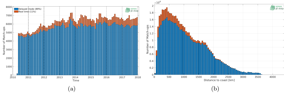
Figure 1: Number of match-ups between Argo and SMOS L4 v2 Weekly (CATDS-CECOS-IFREMER) SSS as a function of time (a) and as function of the distance to coast (b) over the Mid-Low Latitudes 45N-45S Pi-MEP region and for the full satellite product period.
