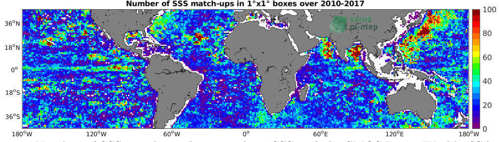
Figure 4: Number of SSS match-ups between Argo SSS and the SMOS L4 v2 Weekly (CATDS-CECOS-IFREMER) SSS product for the Mid-Low Latitudes 45N-45S Pi-MEP region over 1°x1° boxes and for the full satellite product period.
