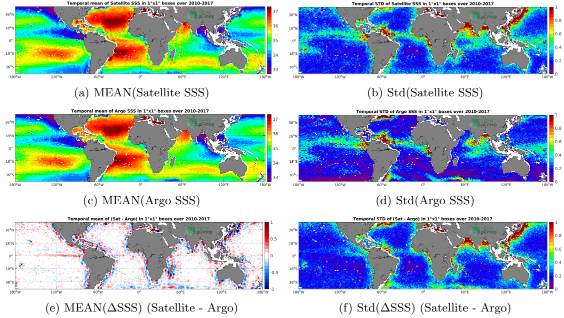
Figure 6: Temporal mean (left) and Std (right) of SSS from SMOS L4 v2 Weekly (CATDS-CECOS-IFREMER) (top), Argo (middle), and of \Delta SSS (Satellite - Argo). Only match-up pairs are used to generate these maps.
