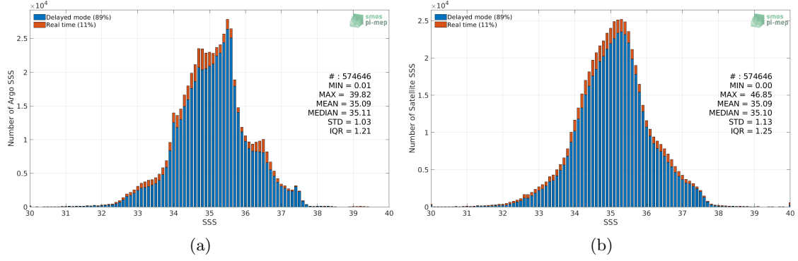
Figure 2: Histograms of SSS from Argo (a) and SMOS L4 v2 Weekly (CATDS-CECOS-IFREMER) (b) considering all match-up pairs per bins of 0.1 over the Mid-Low Latitudes 45N-45S Pi-MEP region and for the full satellite product period.
