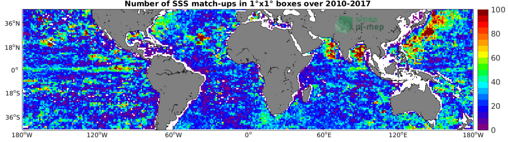
Figure 4: Number of SSS match-ups between Argo SSS and the SMOS L4 v2 Weekly (CATDS-CECOS-IFREMER) SSS product for the Mid-Low Latitudes 45N-45S Pi-MEP region over 1^\circ \times 1^\circ boxes and for the full satellite product period.
