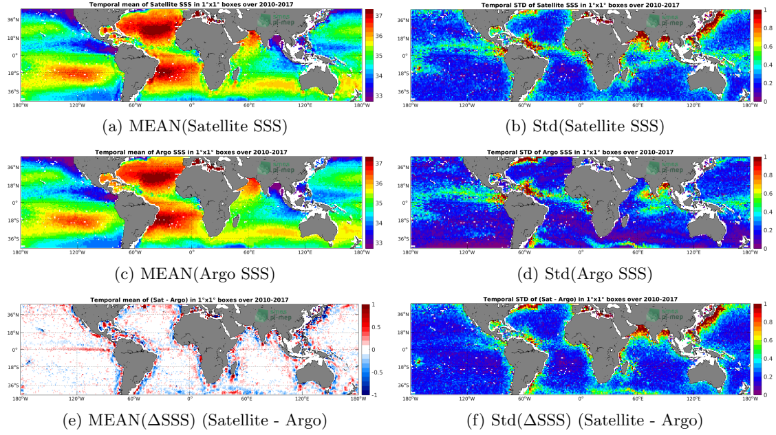
Figure 6: Temporal mean (left) and Std (right) of SSS from SMOS L4 v2 Weekly (CATDS-CECOS-IFREMER) (top), Argo (middle), and of \Delta SSS (Satellite - Argo). Only match-up pairs are used to generate these maps.
