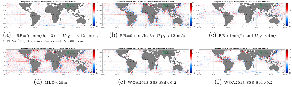
Figure 12: Temporal mean gridded over spatial boxes of size 1^\circ \times 1^\circ of \Delta SSS (SMOS-L4-CATDS-CECOS-IFREMER-V2-WEEKLY-0.5DEG - Argo) for 6 different subdatasets corresponding to:RR=0 mm/h, 3 < U_{10} < 12 m/s, SST >5^\circ\text{C} , distance to coast > 800 km (a), RR=0 mm/h, 3 < U_{10} < 12 m/s (b), RR >1 mm/h and U_{10} < 4 m/s (c),MLD <20 m (d),WOA2013 SSS Std <0.2 (e),WOA2013 SSS Std >0.2 (f).
