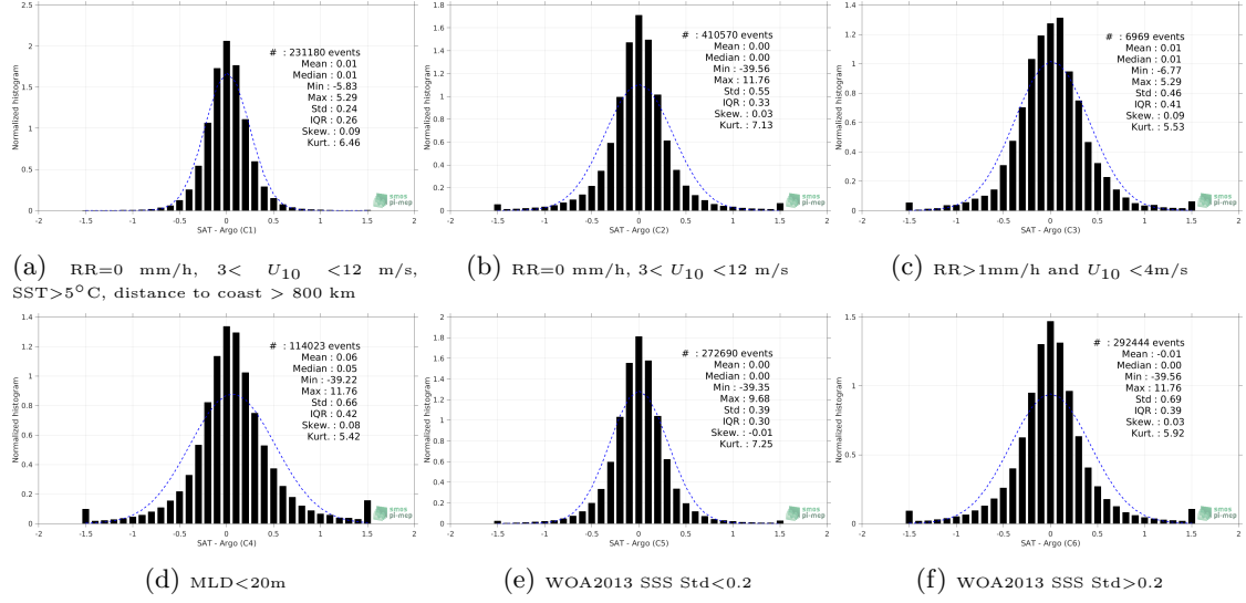
Figure 13: Normalized histogram of \Delta SSS (SMOS-L4-CATDS-CECOS-IFREMER-V2-WEEKLY-0.5DEG - Argo) for 6 different subdatasets corresponding to: RR=0 mm/h, 3 < U_{10} < 12 m/s, SST > 5^\circ C , distance to coast > 800 km (a), RR=0 mm/h, 3 < U_{10} < 12 m/s (b), RR > 1 mm/h and U_{10} < 4 m/s (c), MLD < 20 m (d), WOA2013 SSS Std < 0.2 (e), WOA2013 SSS Std > 0.2 (f).
