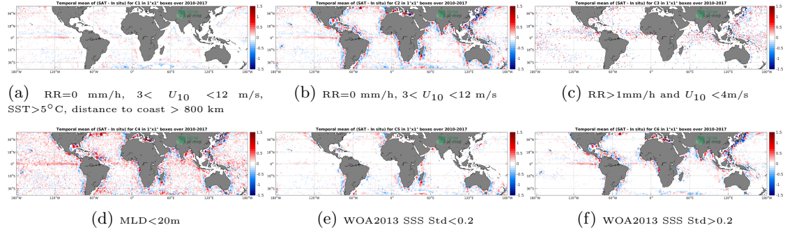
Figure 12: Temporal mean gridded over spatial boxes of size 1^\circ \times 1^\circ of \Delta SSS (SMOS-L4-CATDS-CECOS-IFREMER-V2-WEEKLY-0.5DEG - Argo) for 6 different subdatasets corresponding to: RR=0 mm/h, 3 < U_{10} < 12 m/s, SST > 5^\circ C , distance to coast > 800 km (a), RR=0 mm/h, 3 < U_{10} < 12 m/s (b), RR > 1 mm/h and U_{10} < 4 m/s (c), MLD < 20 m (d), WOA2013 SSS Std < 0.2 (e), WOA2013 SSS Std > 0.2 (f).
