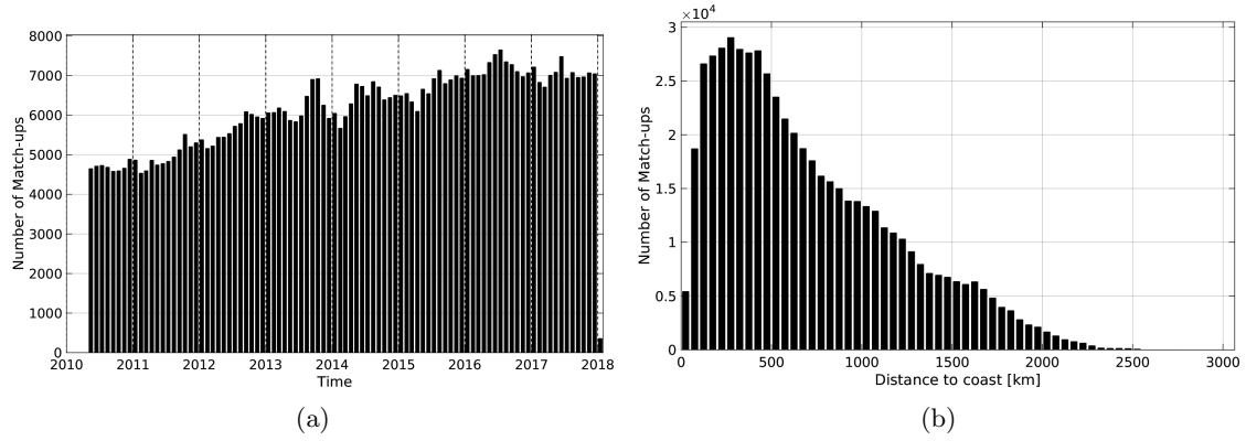
Figure 1: Number of match-ups between Argo and SMOS-L4-CATDS-CECOS-IFREMER-V2-WEEKLY-0.5DEG SSS as a function of time (a) and as function of the distance to coast (b) over the Mid-Low Latitudes 45N-45S Pi-MEP region and for the full satellite product period.
