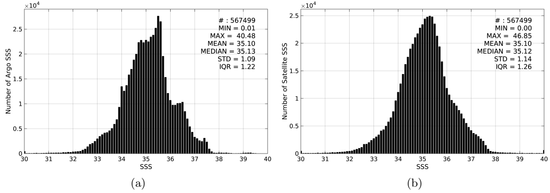
Figure 2: Histograms of SSS from Argos (a) and SMOS-L4-CATDS-CECOS-IFREMER-V2-WEEKLY-0.5DEG (b) considering all match-up pairs per bins of 0.1 over the Mid-Low Latitudes 45N-45S Pi-MEP region and for the full satellite product period.
