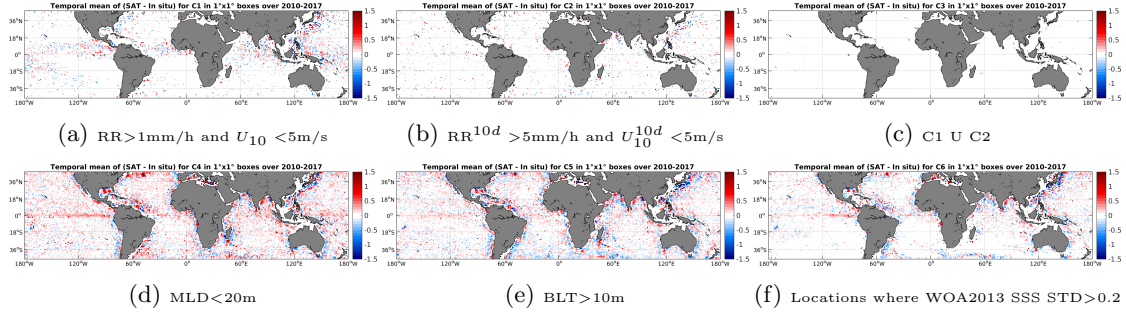
Figure 12: Temporal mean gridded over spatial boxes of size 1^\circ \times 1^\circ of \Delta SSS (SMOS-L4-CATDS-CECOS-IFREMER-V2-WEEKLY-0.5DEG - Argo) for 6 different subdatasets corresponding to: RR > 1\text{mm/h} and U_{10} < 5\text{m/s} (a), RR^{10d} > 5\text{mm/h} and U_{10}^{10d} < 5\text{m/s} (b), C1 U C2 (c), MLD < 20\text{m} (d), BLT > 10\text{m} (e), Locations where WOA2013 SSS STD > 0.2 (f).
