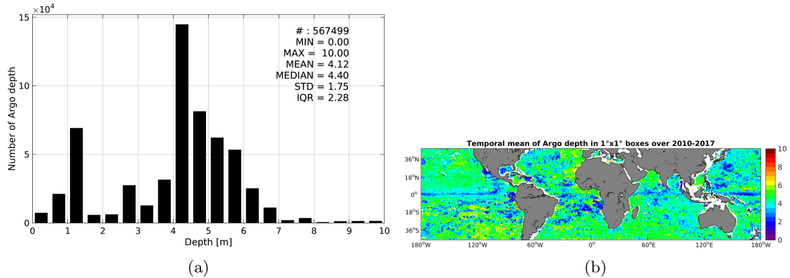
Figure 3: Histograms of the depth of the upper level SSS measurements from Argos in the Match-up DataBase for the Mid-Low Latitudes 45N-45S Pi-MEP region (a) and temporal mean spatial distribution of pressure of the in situ SSS data over 1^\circ \times 1^\circ boxes and for the full satellite product period (b).
