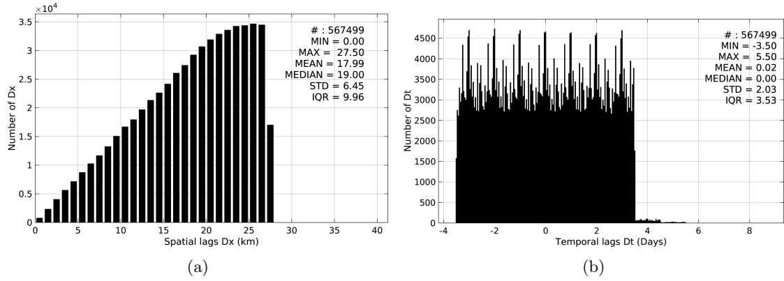
Figure 5: Histograms of the spatial (a) and temporal (b) lags between the time of the Argo measurements and the date of the corresponding SMOS-L4-CATDS-CECOS-IFREMER-V2-WEEKLY-0.5DEG SSS product.
