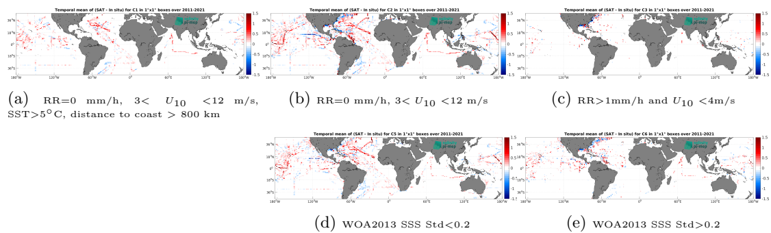
Figure 14: Temporal mean gridded over spatial boxes of size 1^\circ \times 1^\circ of \Delta\text{SSS} (SMOS SSS L4 v2 - Daily (BEC) - TSG (SAMOS)) for 5 different subdatasets corresponding to:RR=0 mm/h, 3 < U_{10} < 12 m/s, SST > 5^\circ\text{C} , distance to coast > 800 km (a), RR=0 mm/h, 3 < U_{10} < 12 m/s (b), RR > 1 mm/h and U_{10} < 4 m/s (c), WOA2013 SSS Std < 0.2 (d), WOA2013 SSS Std > 0.2 (e).
