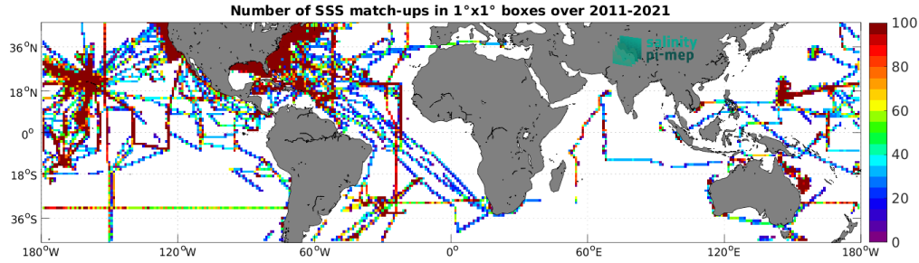
Figure 4: Number of SSS match-ups between TSG (SAMOS) SSS and the SMOS SSS L4 v2 - Daily (BEC) SSS product for the Mid-Low Latitudes 45N-45S Pi-MEP region over 1^\circ \times 1^\circ boxes and for the full satellite product period.
