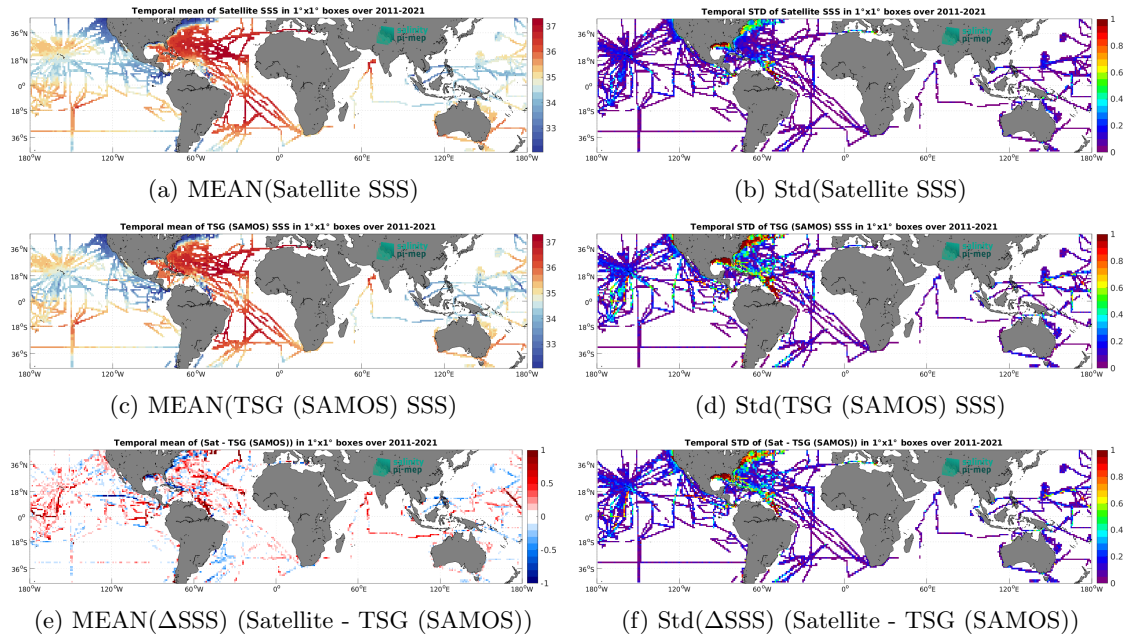
Figure 6: Temporal mean (left) and Std (right) of SSS from SMOS SSS L4 v2 - Daily (BEC) (top), TSG (SAMOS) (middle), and of \Delta SSS (Satellite - TSG (SAMOS)). Only match-up pairs are used to generate these maps.
