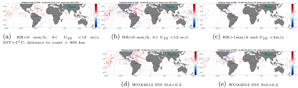
Figure 12: Temporal mean gridded over spatial boxes of size 1^\circ \times 1^\circ of \Delta SSS (SMOS SSS L4 v2 - Daily (BEC) - TSG (SAMOS)) for 5 different subdatasets corresponding to:RR=0 mm/h, 3 < U_{10} < 12 m/s, SST >5^\circ\text{C} , distance to coast > 800 km (a), RR=0 mm/h, 3 < U_{10} < 12 m/s (b), RR >1 mm/h and U_{10} < 4 m/s (c), WOA2013 SSS Std <0.2 (d), WOA2013 SSS Std >0.2 (e).
