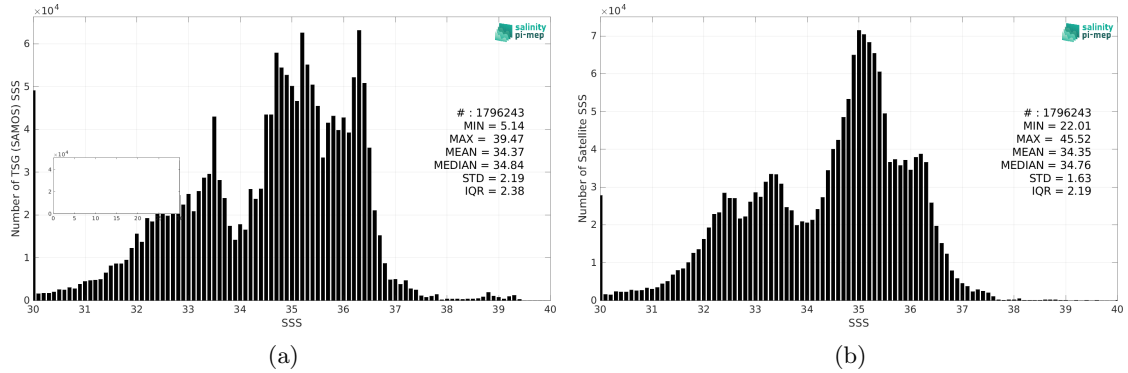
Figure 2: Histograms of SSS from TSG (SAMOS) (a) and SMOS SSS L4 v2 - Daily (BEC) (b) considering all match-up pairs per bins of 0.1 over the Mid-Low Latitudes 45N-45S Pi-MEP region and for the full satellite product period.
