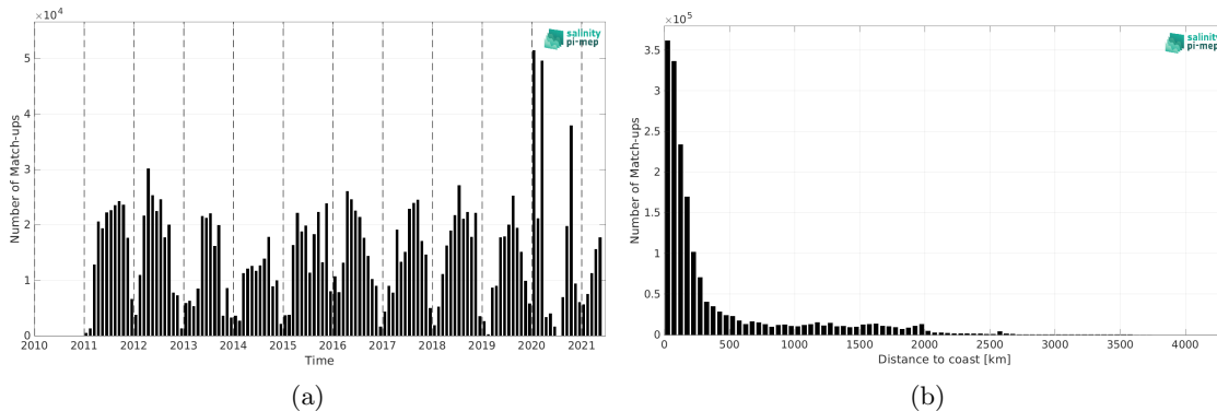
Figure 1: Number of match-ups between TSG (SAMOS) and SMOS SSS L4 v2 - Daily (BEC) SSS as a function of time (a) and as function of the distance to coast (b) over the Mid-Low Latitudes 45N-45S Pi-MEP region and for the full satellite product period.
