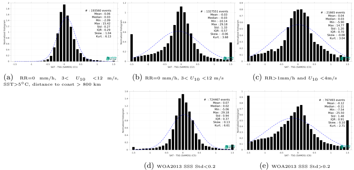
Figure 13: Normalized histogram of \Delta SSS (SMOS SSS L4 v2 - Daily (BEC) - TSG (SAMOS)) for 5 different subdatasets corresponding to: RR=0 mm/h, 3 < U_{10} < 12 m/s, SST >5^\circ\text{C} , distance to coast > 800 km (a), RR=0 mm/h, 3 < U_{10} < 12 m/s (b), RR >1 mm/h and U_{10} < 4 m/s (c), WOA2013 SSS Std <0.2 (d), WOA2013 SSS Std >0.2 (e).
