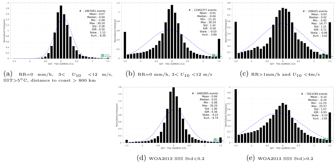
Figure 13: Normalized histogram of \Delta\text{SSS} (SMOS SSS L4 v2 - Daily (BEC) - TSG (SAMOS)) for 5 different subdatasets corresponding to: RR=0 mm/h, 3 < U_{10} < 12 m/s, SST >5^\circ\text{C} , distance to coast > 800 km (a), RR=0 mm/h, 3 < U_{10} < 12 m/s (b), RR >1 mm/h and U_{10} < 4 m/s (c), WOA2013 SSS Std <0.2 (d), WOA2013 SSS Std >0.2 (e).
