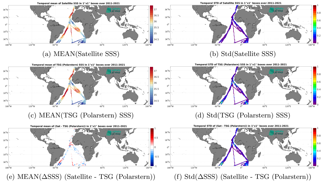
Figure 7: Temporal mean (left) and Std (right) of SSS from SMOS SSS L4 v2 - Daily (BEC) (top), TSG (Polarstern) (middle), and of \Delta SSS (Satellite - TSG (Polarstern)). Only match-up pairs are used to generate these maps.
