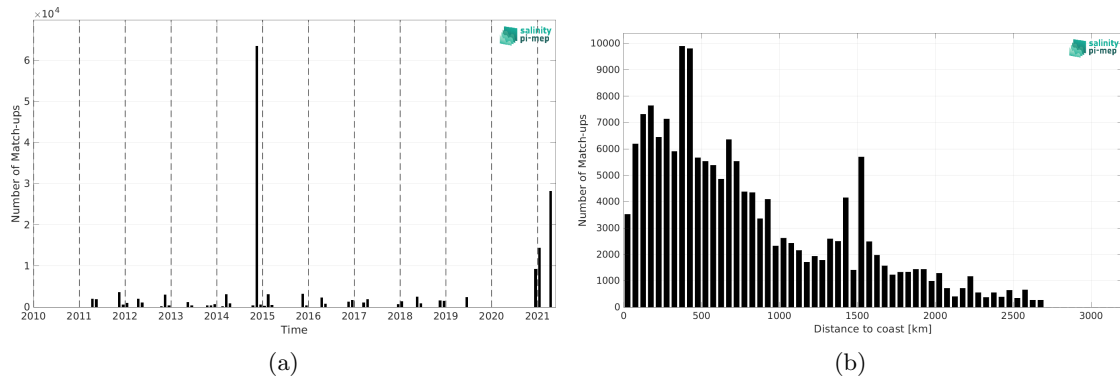
Figure 2: Number of match-ups between TSG (Polarstern) and SMOS SSS L4 v2 - Daily (BEC) SSS as a function of time (a) and as function of the distance to coast (b) over the Mid-Low Latitudes 45N-45S Pi-MEP region and for the full satellite product period.
