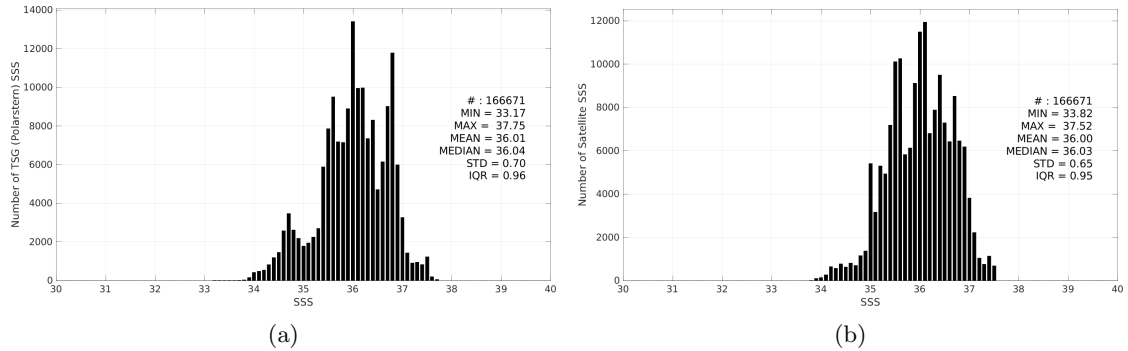
Figure 3: Histograms of SSS from TSG (Polarstern) (a) and SMOS SSS L4 v2 - Daily (BEC) (b) considering all match-up pairs per bins of 0.1 over the Mid-Low Latitudes 45N-45S Pi-MEP region and for the full satellite product period.
