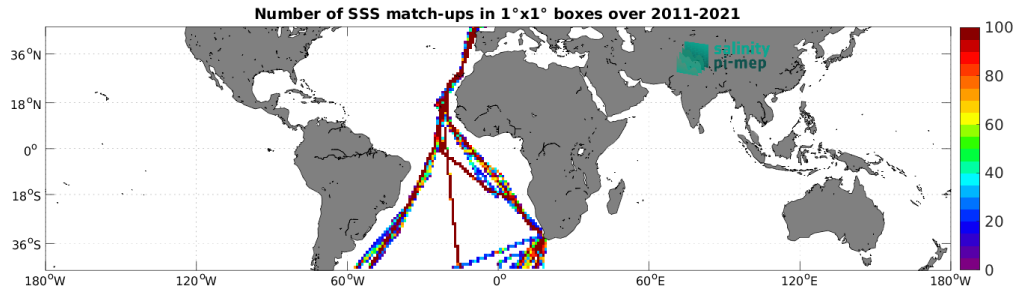
Figure 5: Number of SSS match-ups between TSG (Polarstern) SSS and the SMOS SSS L4 v2 - Daily (BEC) SSS product for the Mid-Low Latitudes 45N-45S Pi-MEP region over 1^\circ \times 1^\circ boxes and for the full satellite product period.
