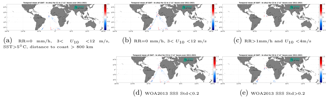
Figure 12: Temporal mean gridded over spatial boxes of size 1^\circ \times 1^\circ of \Delta SSS (SMOS SSS L4 v2 - Daily (BEC) - TSG (Polarstern)) for 5 different subdatasets corresponding to:RR=0 mm/h, 3 < U_{10} < 12 m/s, SST >5^\circ\text{C} , distance to coast > 800 km (a), RR=0 mm/h, 3 < U_{10} < 12 m/s (b), RR >1 mm/h and U_{10} < 4 m/s (c), WOA2013 SSS Std <0.2 (d), WOA2013 SSS Std >0.2 (e).
