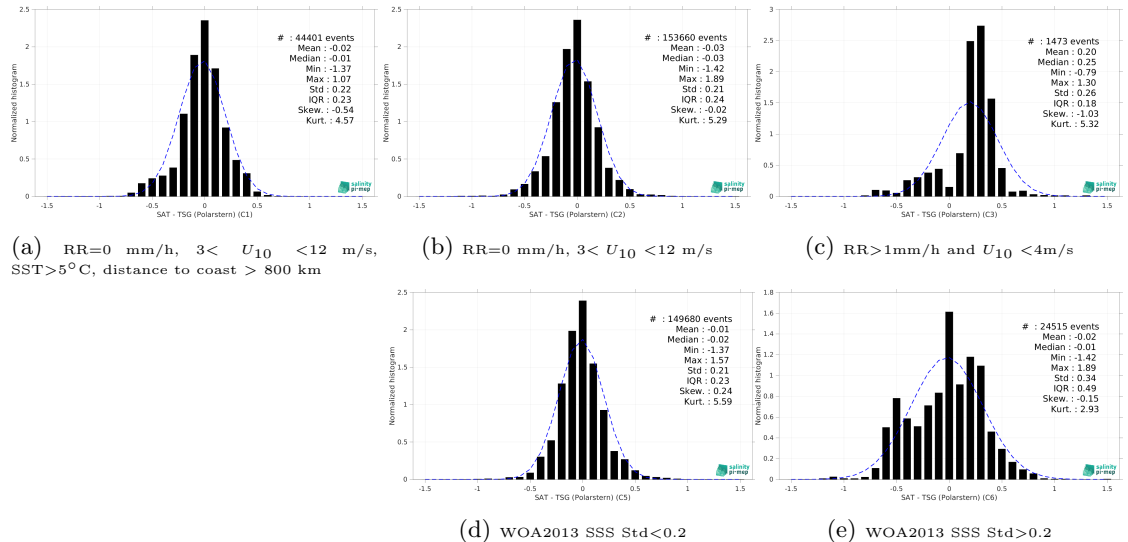
Figure 13: Normalized histogram of \Delta SSS (SMOS SSS L4 v2 - Daily (BEC) - TSG (Polarstern)) for 5 different subdatasets corresponding to: RR=0 mm/h, 3 < U_{10} < 12 m/s, SST >5^\circ\text{C} , distance to coast > 800 km (a), RR=0 mm/h, 3 < U_{10} < 12 m/s (b), RR >1 mm/h and U_{10} < 4 m/s (c), WOA2013 SSS Std <0.2 (d), WOA2013 SSS Std >0.2 (e).
