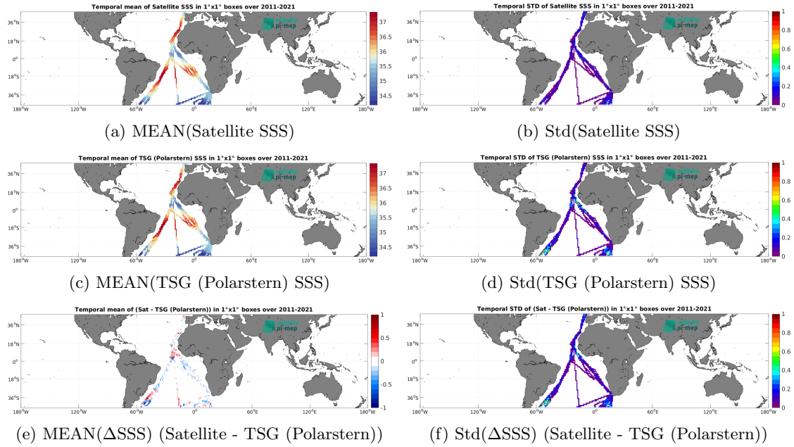
Figure 6: Temporal mean (left) and Std (right) of SSS from SMOS SSS L4 v2 - Daily (BEC) (top), TSG (Polarstern) (middle), and of \Delta SSS (Satellite - TSG (Polarstern)). Only match-up pairs are used to generate these maps.
