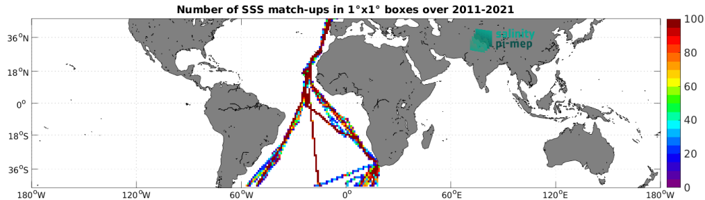
Figure 4: Number of SSS match-ups between TSG (Polarstern) SSS and the SMOS SSS L4 v2 - Daily (BEC) SSS product for the Mid-Low Latitudes 45N-45S Pi-MEP region over 1^\circ \times 1^\circ boxes and for the full satellite product period.
