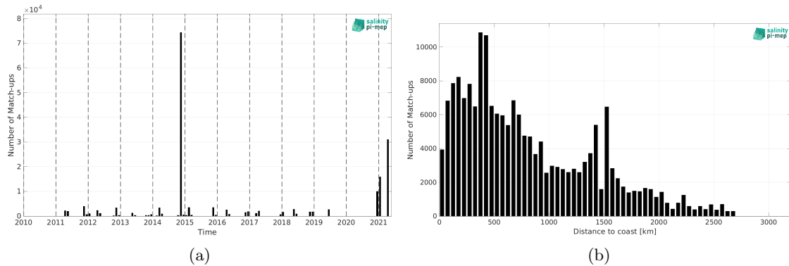
Figure 1: Number of match-ups between TSG (Polarstern) and SMOS SSS L4 v2 - Daily (BEC) SSS as a function of time (a) and as function of the distance to coast (b) over the Mid-Low Latitudes 45N-45S Pi-MEP region and for the full satellite product period.
