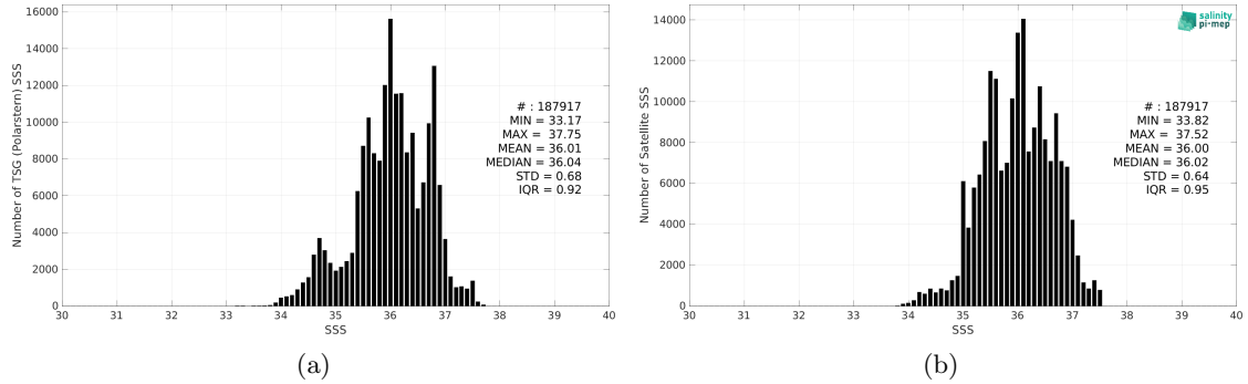
Figure 2: Histograms of SSS from TSG (Polarstern) (a) and SMOS SSS L4 v2 - Daily (BEC) (b) considering all match-up pairs per bins of 0.1 over the Mid-Low Latitudes 45N-45S Pi-MEP region and for the full satellite product period.
