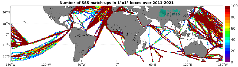
Figure 5: Number of SSS match-ups between TSG (LEGOS-DM) SSS and the SMOS SSS L4 v2 - Daily (BEC) SSS product for the Mid-Low Latitudes 45N-45S Pi-MEP region over 1^\circ \times 1^\circ boxes and for the full satellite product period.
