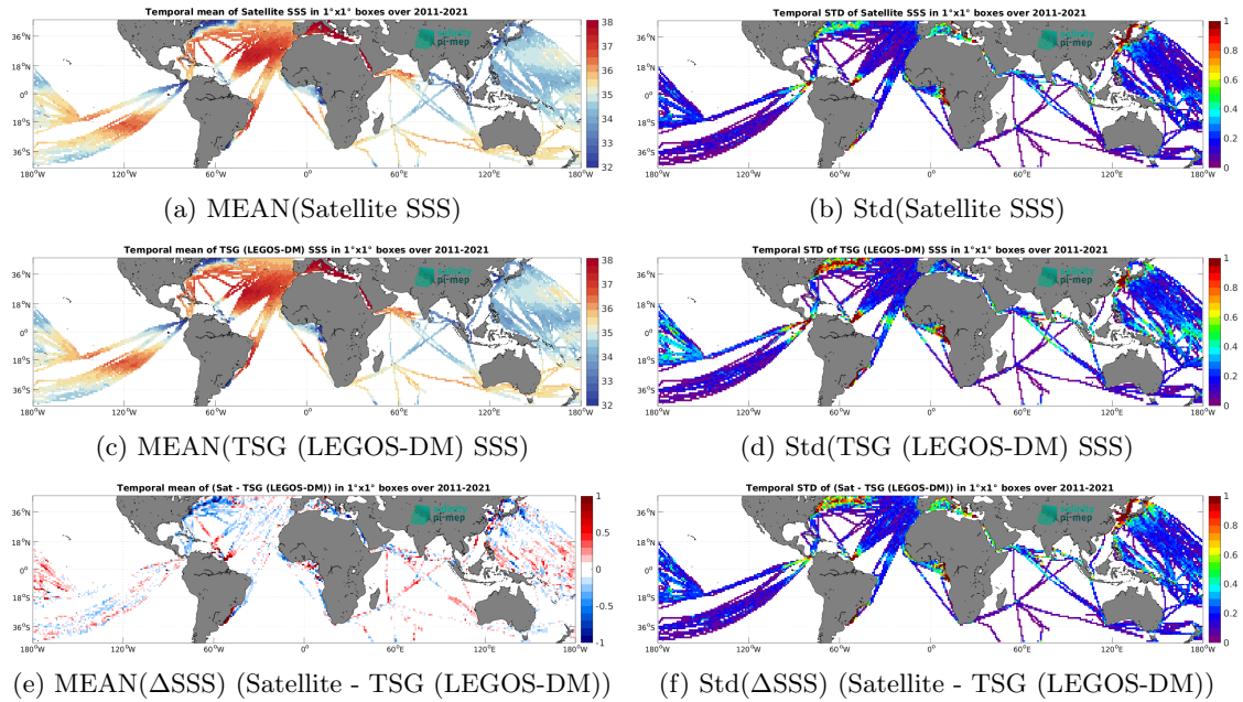
Figure 7: Temporal mean (left) and Std (right) of SSS from SMOS SSS L4 v2 - Daily (BEC) (top), TSG (LEGOS-DM) (middle), and of \Delta SSS (Satellite - TSG (LEGOS-DM)). Only match-up pairs are used to generate these maps.
