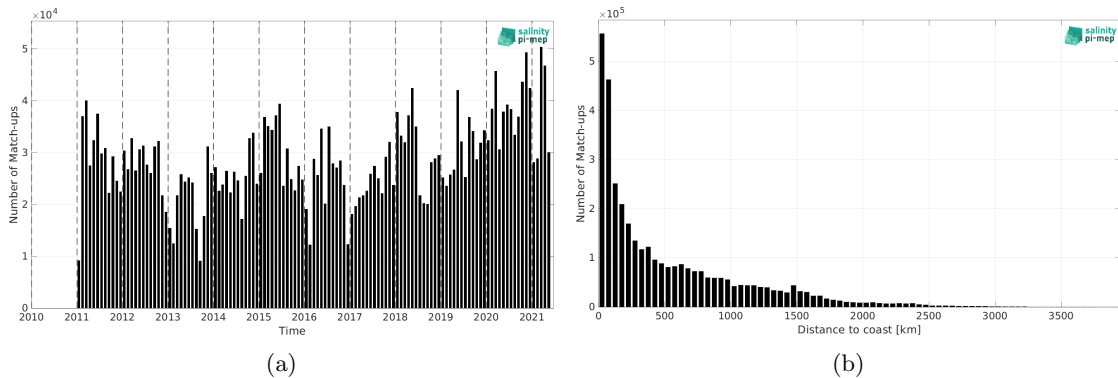
Figure 2: Number of match-ups between TSG (LEGOS-DM) and SMOS SSS L4 v2 - Daily (BEC) SSS as a function of time (a) and as function of the distance to coast (b) over the Mid-Low Latitudes 45N-45S Pi-MEP region and for the full satellite product period.
