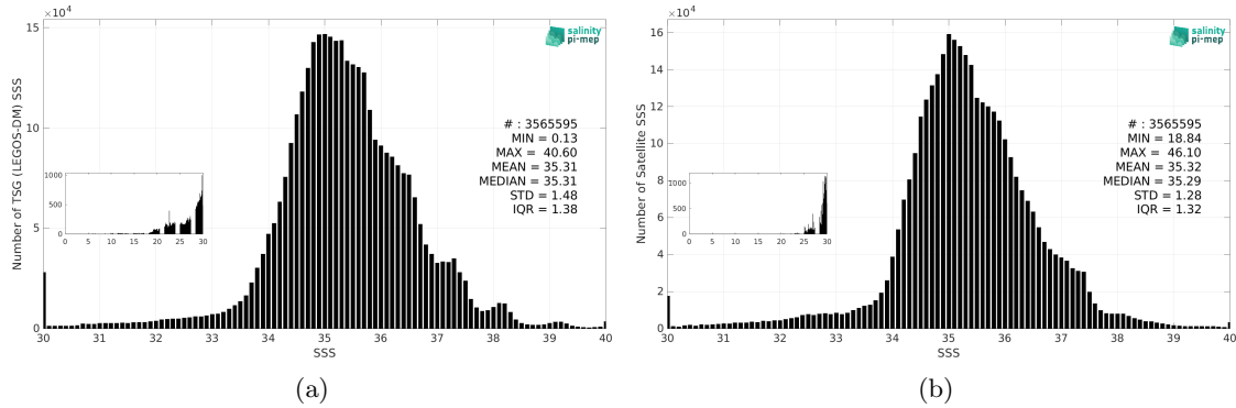
Figure 3: Histograms of SSS from TSG (LEGOS-DM) (a) and SMOS SSS L4 v2 - Daily (BEC) (b) considering all match-up pairs per bins of 0.1 over the Mid-Low Latitudes 45N-45S Pi-MEP region and for the full satellite product period.
