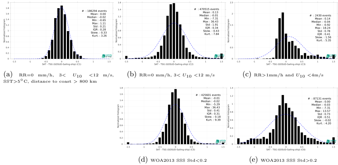
Figure 15: Normalized histogram of \Delta\text{SSS} (SMOS SSS L4 v2 - Daily (BEC) - TSG (GOSUD-Sailing-ship)) for 5 different subdatasets corresponding to: RR=0 mm/h, 3 < U_{10} < 12 m/s, SST > 5^{\circ}\text{C} , distance to coast > 800 km (a), RR=0 mm/h, 3 < U_{10} < 12 m/s (b), RR > 1 mm/h and U_{10} < 4 m/s (c), WOA2013 SSS Std < 0.2 (d), WOA2013 SSS Std > 0.2 (e).
