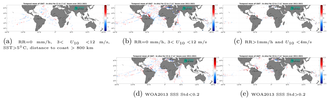
Figure 14: Temporal mean gridded over spatial boxes of size 1^\circ \times 1^\circ of \Delta\text{SSS} (SMOS SSS L4 v2 - Daily (BEC) - TSG (GOSUD-Research-vessel)) for 5 different subdatasets corresponding to: RR=0 mm/h, 3 < U_{10} < 12 m/s, SST > 5°C, distance to coast > 800 km (a), RR=0 mm/h, 3 < U_{10} < 12 m/s (b), RR > 1mm/h and U_{10} < 4 m/s (c), WOA2013 SSS Std < 0.2 (d), WOA2013 SSS Std > 0.2 (e).
