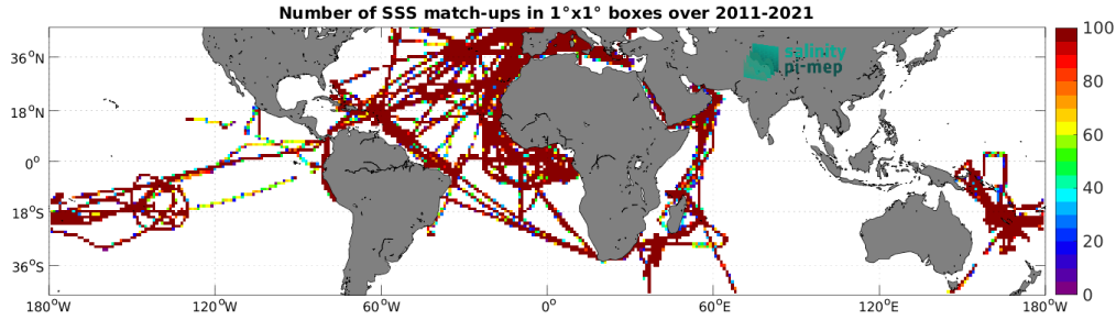
Figure 5: Number of SSS match-ups between TSG (GOSUD-Research-vessel) SSS and the SMOS SSS L4 v2 - Daily (BEC) SSS product for the Mid-Low Latitudes 45N-45S Pi-MEP region over 1^\circ \times 1^\circ boxes and for the full satellite product period.
