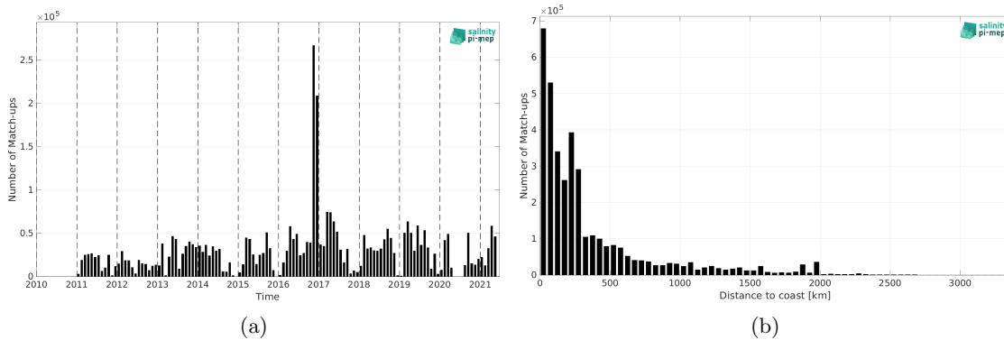
Figure 2: Number of match-ups between TSG (GOSUD-Research-vessel) and SMOS SSS L4 v2 - Daily (BEC) SSS as a function of time (a) and as function of the distance to coast (b) over the Mid-Low Latitudes 45N-45S Pi-MEP region and for the full satellite product period.
