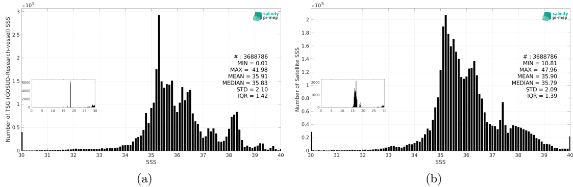
Figure 3: Histograms of SSS from TSG (GOSUD-Research-vessel) (a) and SMOS SSS L4 v2 - Daily (BEC) (b) considering all match-up pairs per bins of 0.1 over the Mid-Low Latitudes 45N-45S Pi-MEP region and for the full satellite product period.
