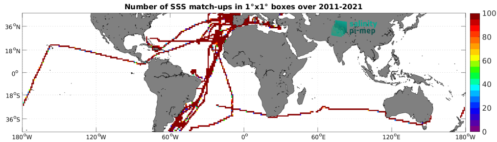
Figure 5: Number of SSS match-ups between TSG (CSIC-UTM) SSS and the SMOS SSS L4 v2 - Daily (BEC) SSS product for the Mid-Low Latitudes 45N-45S Pi-MEP region over 1^\circ \times 1^\circ boxes and for the full satellite product period.
