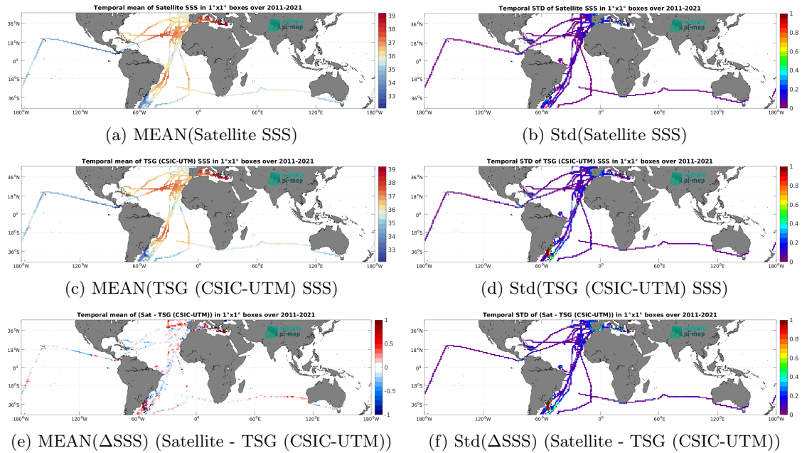
Figure 7: Temporal mean (left) and Std (right) of SSS from SMOS SSS L4 v2 - Daily (BEC) (top), TSG (CSIC-UTM) (middle), and of \Delta SSS (Satellite - TSG (CSIC-UTM)). Only match-up pairs are used to generate these maps.
