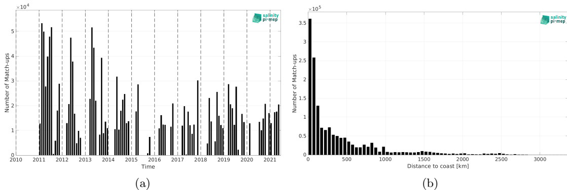
Figure 2: Number of match-ups between TSG (CSIC-UTM) and SMOS SSS L4 v2 - Daily (BEC) SSS as a function of time (a) and as function of the distance to coast (b) over the Mid-Low Latitudes 45N-45S Pi-MEP region and for the full satellite product period.
