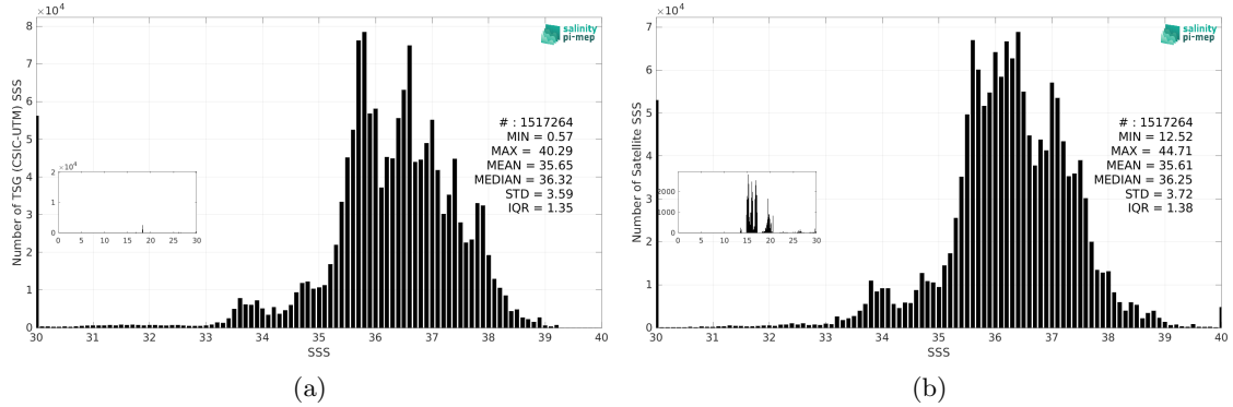
Figure 3: Histograms of SSS from TSG (CSIC-UTM) (a) and SMOS SSS L4 v2 - Daily (BEC) (b) considering all match-up pairs per bins of 0.1 over the Mid-Low Latitudes 45N-45S Pi-MEP region and for the full satellite product period.
