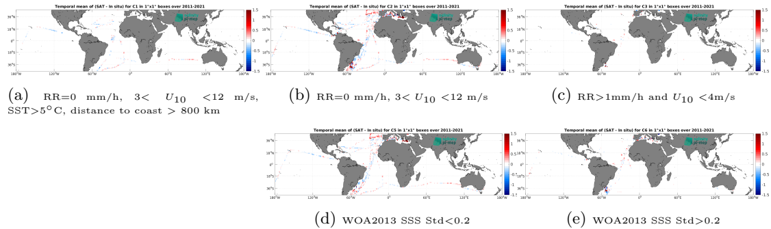
Figure 12: Temporal mean gridded over spatial boxes of size 1^\circ \times 1^\circ of \Delta\text{SSS} (SMOS SSS L4 v2 - Daily (BEC) - TSG (CSIC-UTM)) for 5 different subdatasets corresponding to:RR=0 mm/h, 3 < U_{10} < 12 m/s, SST >5^\circ\text{C} , distance to coast > 800 km (a), RR=0 mm/h, 3 < U_{10} < 12 m/s (b), RR >1 mm/h and U_{10} < 4 m/s (c), WOA2013 SSS Std <0.2 (d), WOA2013 SSS Std >0.2 (e).
