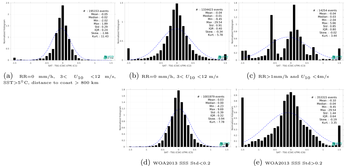
Figure 13: Normalized histogram of \Delta\text{SSS} (SMOS SSS L4 v2 - Daily (BEC) - TSG (CSIC-UTM)) for 5 different subdatasets corresponding to: RR=0 mm/h, 3 < U_{10} < 12 m/s, SST >5^\circ\text{C} , distance to coast > 800 km (a), RR=0 mm/h, 3 < U_{10} < 12 m/s (b), RR >1 mm/h and U_{10} < 4 m/s (c), WOA2013 SSS Std <0.2 (d), WOA2013 SSS Std >0.2 (e).
