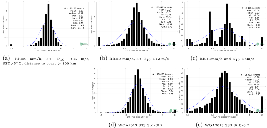
Figure 13: Normalized histogram of \Delta SSS (SMOS SSS L4 v2 - Daily (BEC) - TSG (CSIC-UTM)) for 5 different subdatasets corresponding to: RR=0 mm/h, 3 < U_{10} < 12 m/s, SST >5^\circ C, distance to coast > 800 km (a), RR=0 mm/h, 3 < U_{10} < 12 m/s (b), RR >1 mm/h and U_{10} < 4 m/s (c), WOA2013 SSS Std <0.2 (d), WOA2013 SSS Std >0.2 (e).
