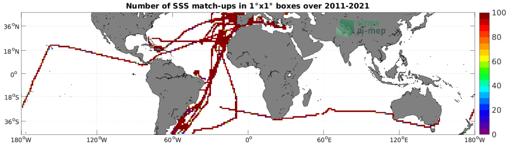
Figure 4: Number of SSS match-ups between TSG (CSIC-UTM) SSS and the SMOS SSS L4 v2 - Daily (BEC) SSS product for the Mid-Low Latitudes 45N-45S Pi-MEP region over 1^\circ \times 1^\circ boxes and for the full satellite product period.
