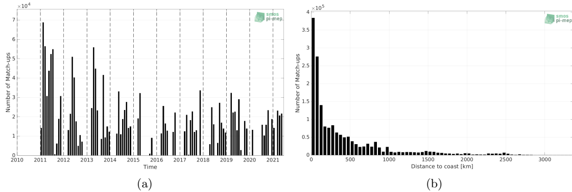
Figure 1: Number of match-ups between TSG (CSIC-UTM) and SMOS SSS L4 v2 - Daily (BEC) SSS as a function of time (a) and as function of the distance to coast (b) over the Mid-Low Latitudes 45N-45S Pi-MEP region and for the full satellite product period.
