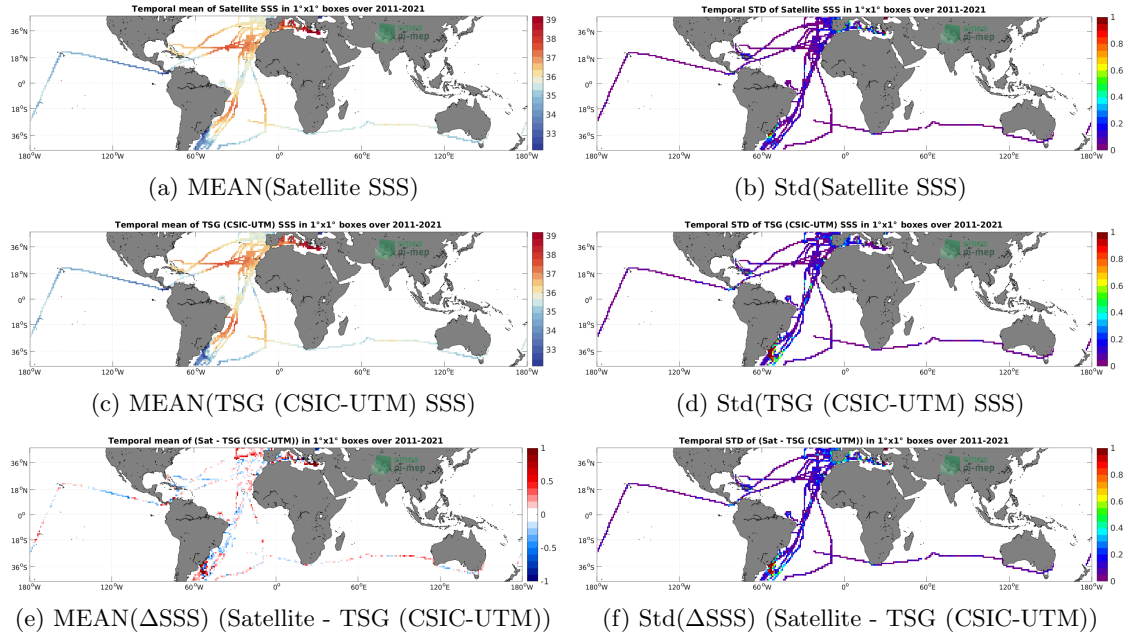
Figure 6: Temporal mean (left) and Std (right) of SSS from SMOS SSS L4 v2 - Daily (BEC) (top), TSG (CSIC-UTM) (middle), and of \Delta SSS (Satellite - TSG (CSIC-UTM)). Only match-up pairs are used to generate these maps.
