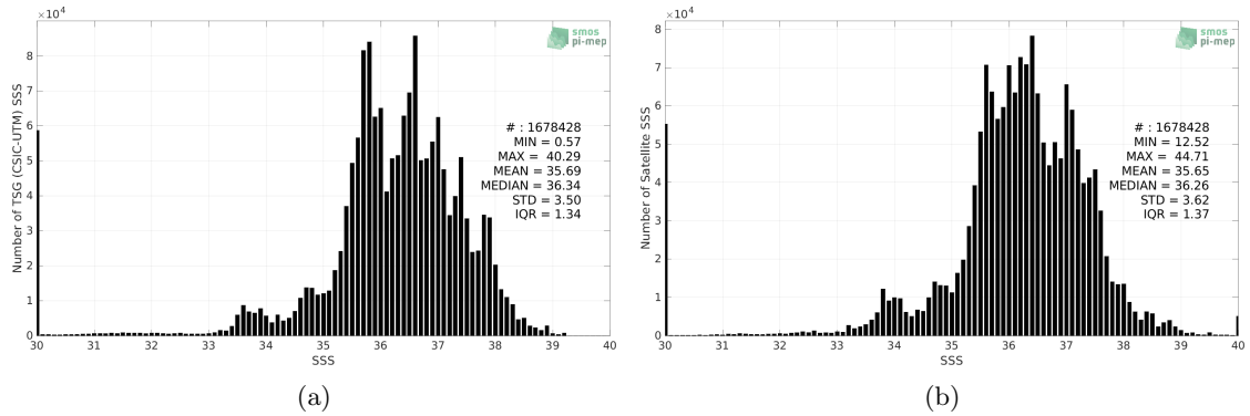
Figure 2: Histograms of SSS from TSG (CSIC-UTM) (a) and SMOS SSS L4 v2 - Daily (BEC) (b) considering all match-up pairs per bins of 0.1 over the Mid-Low Latitudes 45N-45S Pi-MEP region and for the full satellite product period.
