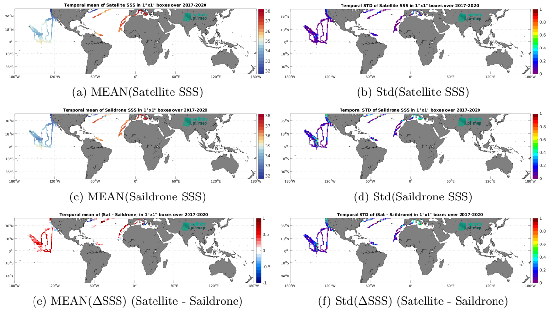
Figure 7: Temporal mean (left) and Std (right) of SSS from SMOS SSS L4 v2 - Daily (BEC) (top), Saildrone (middle), and of \Delta SSS (Satellite - Saildrone). Only match-up pairs are used to generate these maps.
