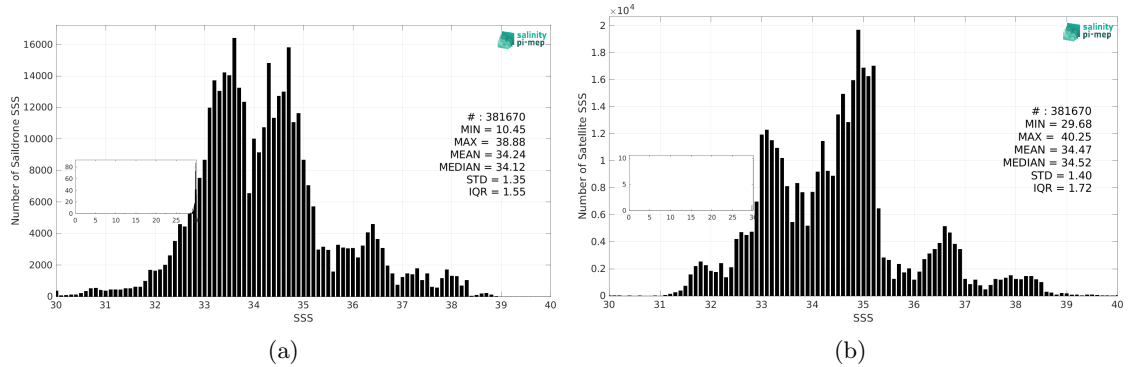
Figure 3: Histograms of SSS from Saildrone (a) and SMOS SSS L4 v2 - Daily (BEC) (b) considering all match-up pairs per bins of 0.1 over the Mid-Low Latitudes 45N-45S Pi-MEP region and for the full satellite product period.
