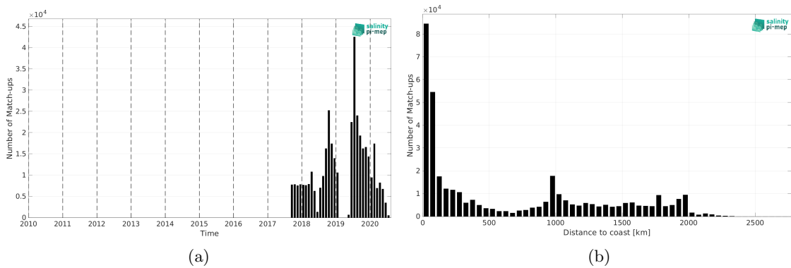
Figure 2: Number of match-ups between Saildrone and SMOS SSS L4 v2 - Daily (BEC) SSS as a function of time (a) and as function of the distance to coast (b) over the Mid-Low Latitudes 45N-45S Pi-MEP region and for the full satellite product period.
