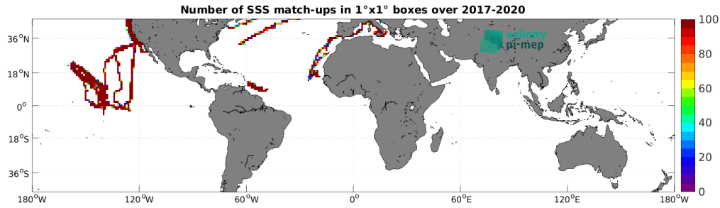
Figure 5: Number of SSS match-ups between Saildrone SSS and the SMOS SSS L4 v2 - Daily (BEC) SSS product for the Mid-Low Latitudes 45N-45S Pi-MEP region over 1^\circ \times 1^\circ boxes and for the full satellite product period.
