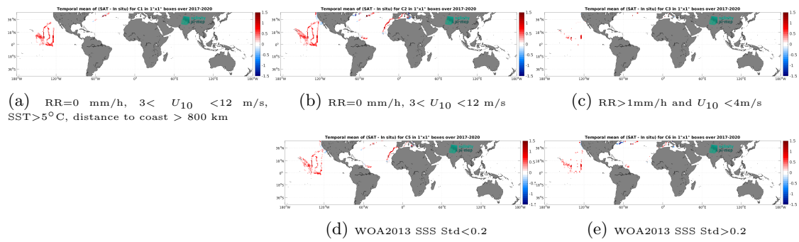
Figure 14: Temporal mean gridded over spatial boxes of size 1^\circ \times 1^\circ of \Delta\text{SSS} (SMOS SSS L4 v2 - Daily (BEC) - Saldrone) for 5 different subdatasets corresponding to:RR=0 mm/h, 3 < U_{10} < 12 m/s, SST>5°C, distance to coast > 800 km (a), RR=0 mm/h, 3 < U_{10} < 12 m/s (b), RR>1mm/h and U_{10} < 4 m/s (c), WOA2013 SSS Std<0.2 (d), WOA2013 SSS Std>0.2 (e).
