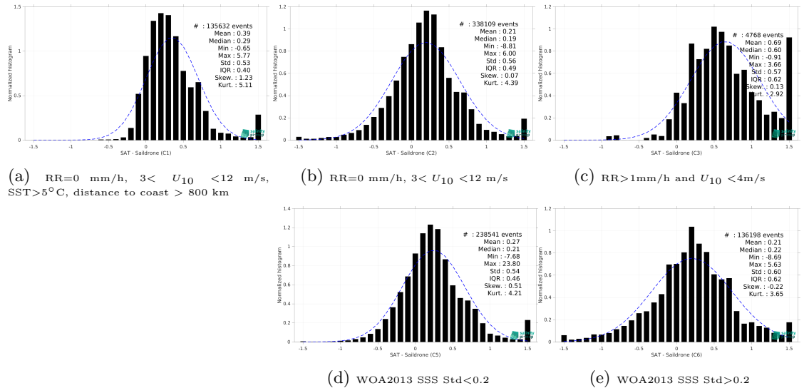
Figure 13: Normalized histogram of \Delta\text{SSS} (SMOS SSS L4 v2 - Daily (BEC) - Saildrone) for 5 different subdatasets corresponding to: RR=0 mm/h, 3 < U_{10} < 12 m/s, SST >5^\circ\text{C} , distance to coast > 800 km (a), RR=0 mm/h, 3 < U_{10} < 12 m/s (b), RR >1 mm/h and U_{10} < 4 m/s (c), WOA2013 SSS Std <0.2 (d), WOA2013 SSS Std >0.2 (e).
