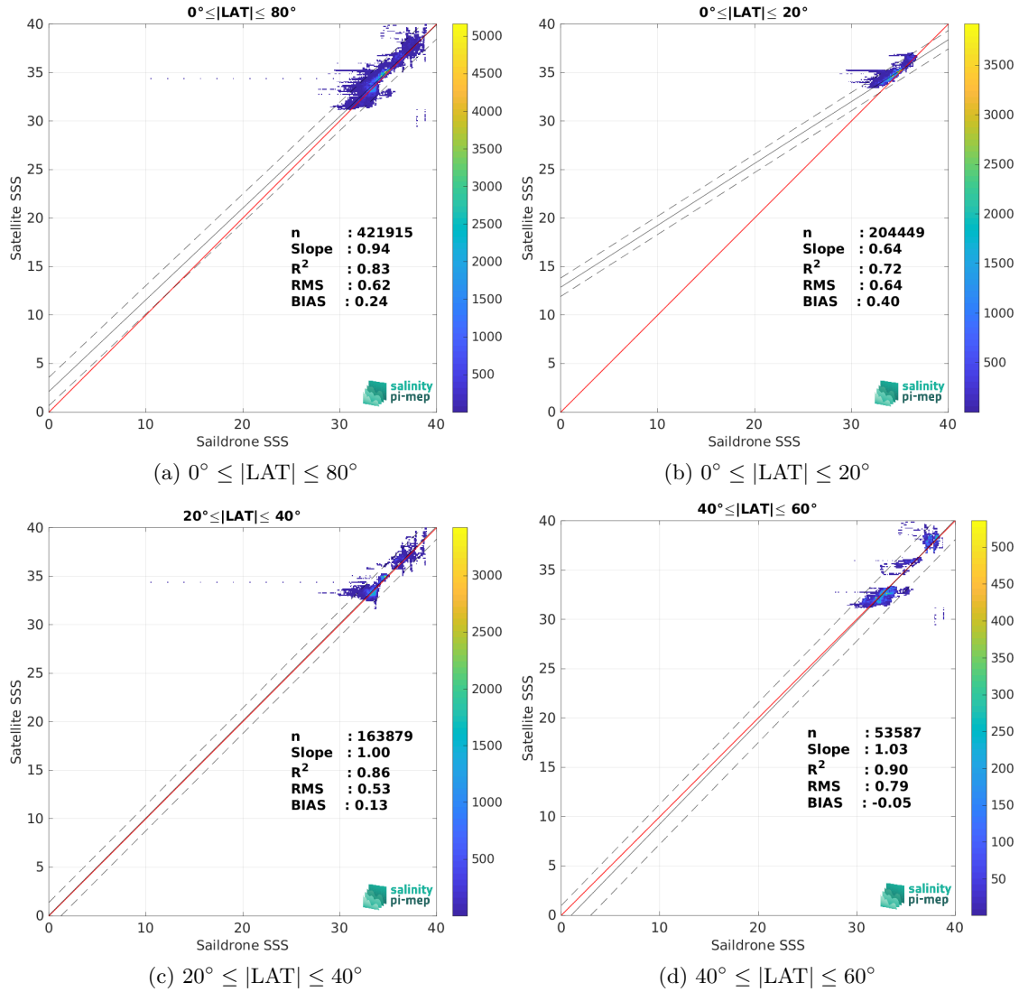
Figure 9: Contour maps of the concentration of SMOS SSS L4 v2 - Daily (BEC) SSS (y-axis) versus Saildrone SSS (x-axis) at match-up pairs for different latitude bands. For each plot, the red line shows x=y . The black thin and dashed lines indicate a linear fit through the data cloud and the \pm 95\% confidence levels, respectively. The number match-up pairs n , the slope and R^2 coefficient of the linear fit, the root mean square (RMS) and the mean bias between satellite and in situ data are indicated for each latitude band in each plots.
