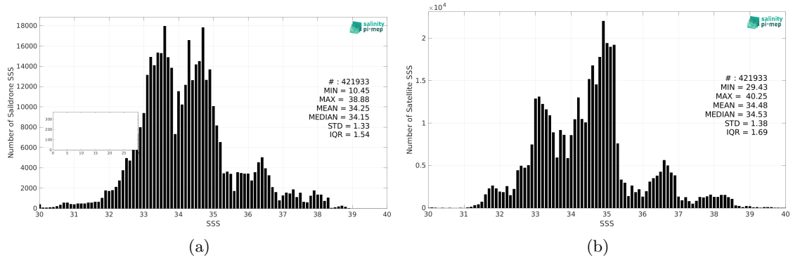
Figure 2: Histograms of SSS from Saildrone (a) and SMOS SSS L4 v2 - Daily (BEC) (b) considering all match-up pairs per bins of 0.1 over the Mid-Low Latitudes 45N-45S Pi-MEP region and for the full satellite product period.
