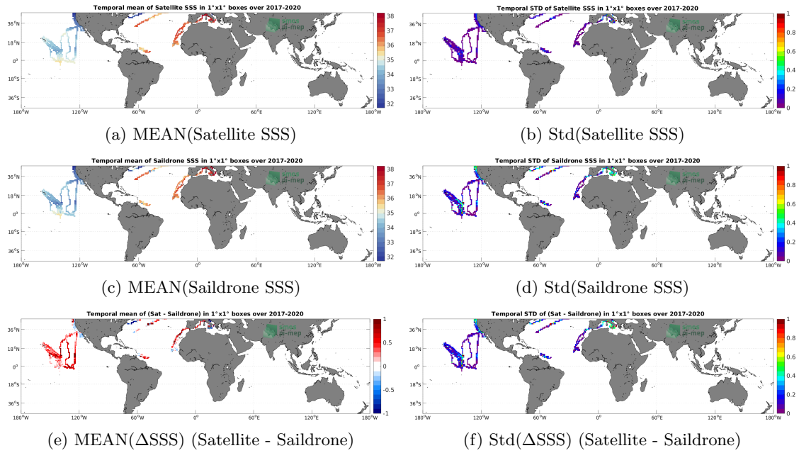
Figure 6: Temporal mean (left) and Std (right) of SSS from SMOS SSS L4 v2 - Daily (BEC) (top), Saildrone (middle), and of \Delta SSS (Satellite - Saildrone). Only match-up pairs are used to generate these maps.
