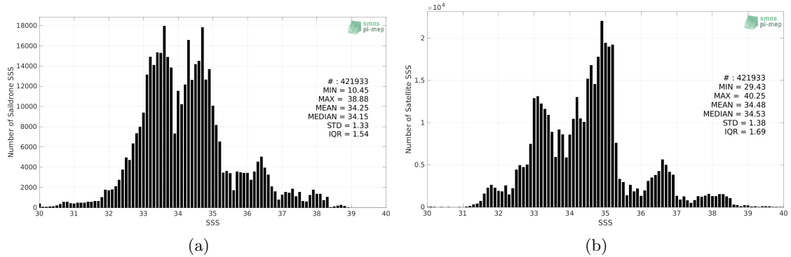
Figure 2: Histograms of SSS from Sairdrone (a) and SMOS SSS L4 v2 - Daily (BEC) (b) considering all match-up pairs per bins of 0.1 over the Mid-Low Latitudes 45N-45S Pi-MEP region and for the full satellite product period.
