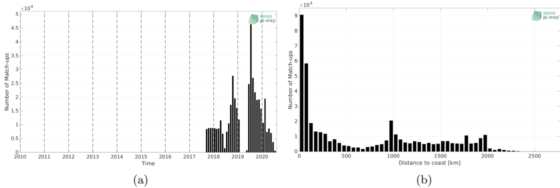
Figure 1: Number of match-ups between Saildrone and SMOS SSS L4 v2 - Daily (BEC) SSS as a function of time (a) and as function of the distance to coast (b) over the Mid-Low Latitudes 45N-45S Pi-MEP region and for the full satellite product period.
