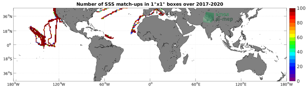
Figure 4: Number of SSS match-ups between Saildrone SSS and the SMOS SSS L4 v2 - Daily (BEC) SSS product for the Mid-Low Latitudes 45N-45S Pi-MEP region over 1^\circ \times 1^\circ boxes and for the full satellite product period.
