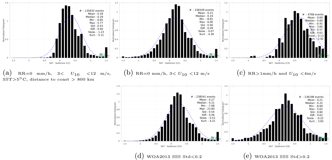
Figure 13: Normalized histogram of \Delta SSS (SMOS SSS L4 v2 - Daily (BEC) - Saildrone) for 5 different subdatasets corresponding to: RR=0 mm/h, 3 < U_{10} < 12 m/s, SST>5°C, distance to coast > 800 km (a), RR=0 mm/h, 3 < U_{10} < 12 m/s (b), RR>1mm/h and U_{10} < 4 m/s (c), WOA2013 SSS Std<0.2 (d), WOA2013 SSS Std>0.2 (e).
