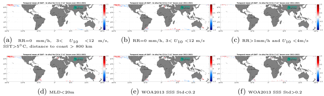
Figure 14: Temporal mean gridded over spatial boxes of size 1^\circ \times 1^\circ of \Delta SSS (SMOS SSS L4 v2 - Daily (BEC) - Marine mammals) for 6 different subdatasets corresponding to:RR=0 mm/h, 3 < U_{10} < 12 m/s, SST>5°C, distance to coast > 800 km (a), RR=0 mm/h, 3 < U_{10} < 12 m/s (b), RR>1mm/h and U_{10} < 4 m/s (c),MLD<20m (d),WOA2013 SSS Std<0.2 (e),WOA2013 SSS Std>0.2 (f).
