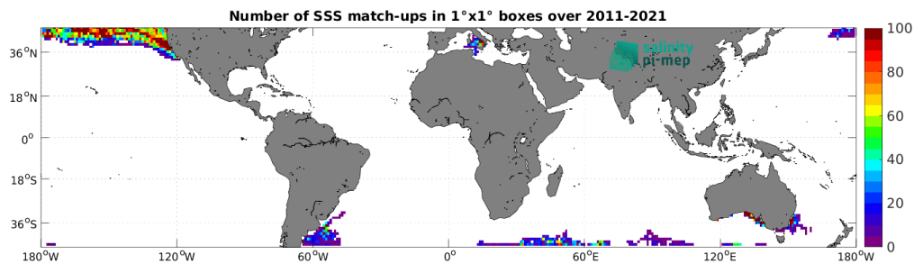
Figure 5: Number of SSS match-ups between Marine mammals SSS and the SMOS SSS L4 v2 - Daily (BEC) SSS product for the Mid-Low Latitudes 45N-45S Pi-MEP region over 1^\circ \times 1^\circ boxes and for the full satellite product period.
