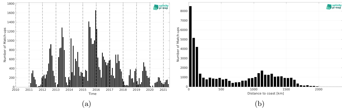
Figure 2: Number of match-ups between Marine mammals and SMOS SSS L4 v2 - Daily (BEC) SSS as a function of time (a) and as function of the distance to coast (b) over the Mid-Low Latitudes 45N-45S Pi-MEP region and for the full satellite product period.
