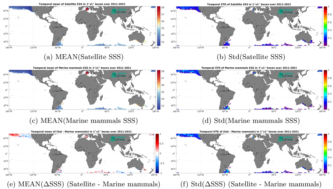
Figure 7: Temporal mean (left) and Std (right) of SSS from SMOS SSS L4 v2 - Daily (BEC) (top), Marine mammals (middle), and of \Delta SSS (Satellite - Marine mammals). Only match-up pairs are used to generate these maps.
