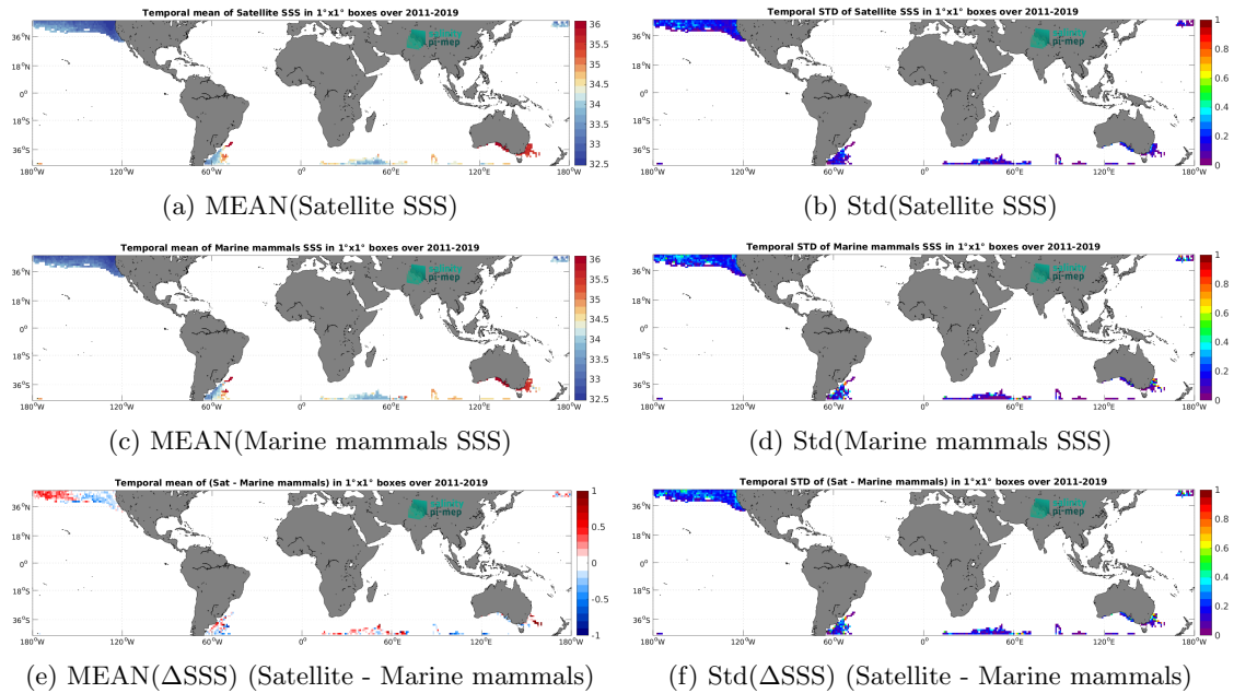
Figure 6: Temporal mean (left) and Std (right) of SSS from SMOS SSS L4 v2 - Daily (BEC) (top), Marine mammals (middle), and of \Delta SSS (Satellite - Marine mammals). Only match-up pairs are used to generate these maps.
