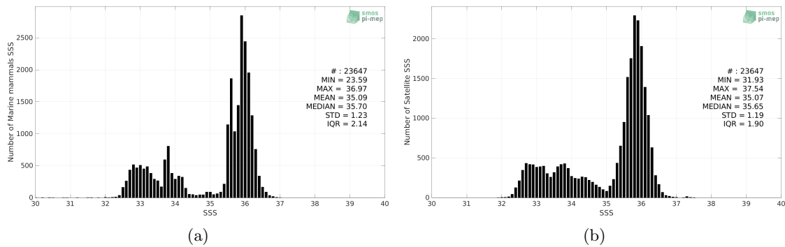
Figure 2: Histograms of SSS from Marine mammals (a) and SMOS SSS L4 v2 - Daily (BEC) (b) considering all match-up pairs per bins of 0.1 over the Mid-Low Latitudes 45N-45S Pi-MEP region and for the full satellite product period.
