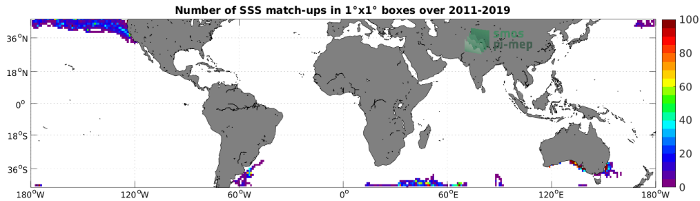
Figure 4: Number of SSS match-ups between Marine mammals SSS and the SMOS SSS L4 v2 - Daily (BEC) SSS product for the Mid-Low Latitudes 45N-45S Pi-MEP region over 1^\circ \times 1^\circ boxes and for the full satellite product period.
