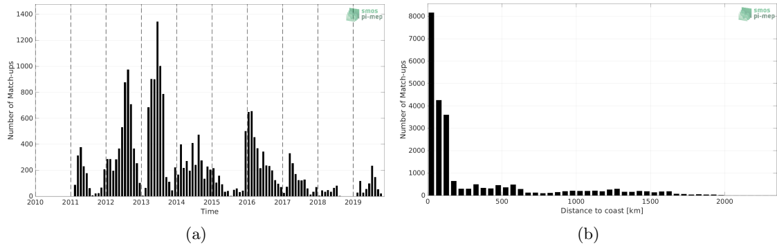
Figure 1: Number of match-ups between Marine mammals and SMOS SSS L4 v2 - Daily (BEC) SSS as a function of time (a) and as function of the distance to coast (b) over the Mid-Low Latitudes 45N-45S Pi-MEP region and for the full satellite product period.
