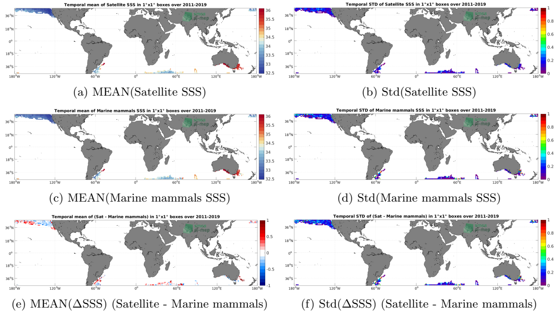
Figure 6: Temporal mean (left) and Std (right) of SSS from SMOS SSS L4 v2 - Daily (BEC) (top), Marine mammals (middle), and of \Delta SSS (Satellite - Marine mammals). Only match-up pairs are used to generate these maps.
