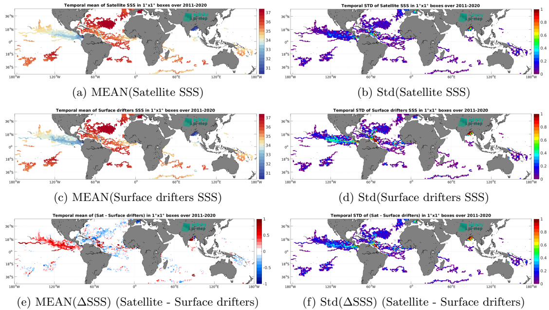
Figure 6: Temporal mean (left) and Std (right) of SSS from SMOS SSS L4 v2 - Daily (BEC) (top), Surface drifters (middle), and of \Delta SSS (Satellite - Surface drifters). Only match-up pairs are used to generate these maps.
