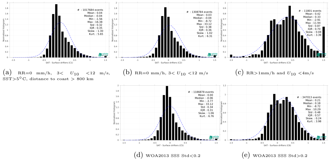
Figure 14: Normalized histogram of \Delta SSS (SMOS SSS L4 v2 - Daily (BEC) - Surface drifters) for 5 different subdatasets corresponding to: RR=0 mm/h, 3 < U_{10} < 12 m/s, SST>5°C, distance to coast > 800 km (a), RR=0 mm/h, 3 < U_{10} < 12 m/s (b), RR>1mm/h and U_{10} < 4 m/s (c), WOA2013 SSS Std<0.2 (d), WOA2013 SSS Std>0.2 (e).
