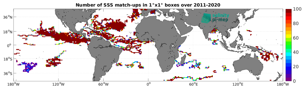
Figure 4: Number of SSS match-ups between Surface drifters SSS and the SMOS SSS L4 v2 - Daily (BEC) SSS product for the Mid-Low Latitudes 45N-45S Pi-MEP region over 1^\circ \times 1^\circ boxes and for the full satellite product period.
