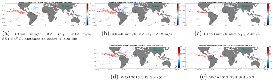
Figure 13: Temporal mean gridded over spatial boxes of size 1^\circ \times 1^\circ of \Delta SSS (SMOS SSS L4 v2 - Daily (BEC) - Surface drifters) for 5 different subdatasets corresponding to: RR=0 mm/h, 3 < U_{10} < 12 m/s, SST>5°C, distance to coast > 800 km (a), RR=0 mm/h, 3 < U_{10} < 12 m/s (b), RR>1mm/h and U_{10} < 4 m/s (c), WOA2013 SSS Std<0.2 (d), WOA2013 SSS Std>0.2 (e).
