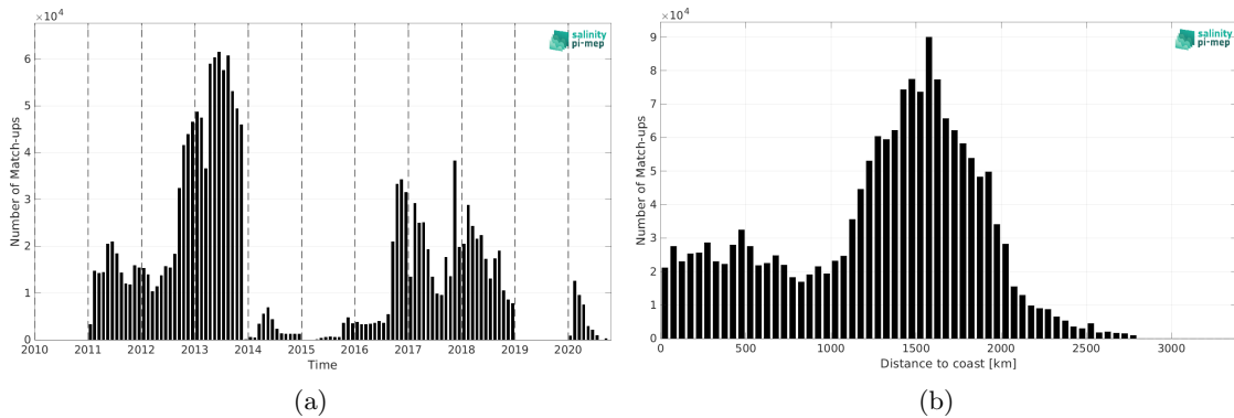
Figure 2: Number of match-ups between Surface drifters and SMOS SSS L4 v2 - Daily (BEC) SSS as a function of time (a) and as function of the distance to coast (b) over the Mid-Low Latitudes 45N-45S Pi-MEP region and for the full satellite product period.
