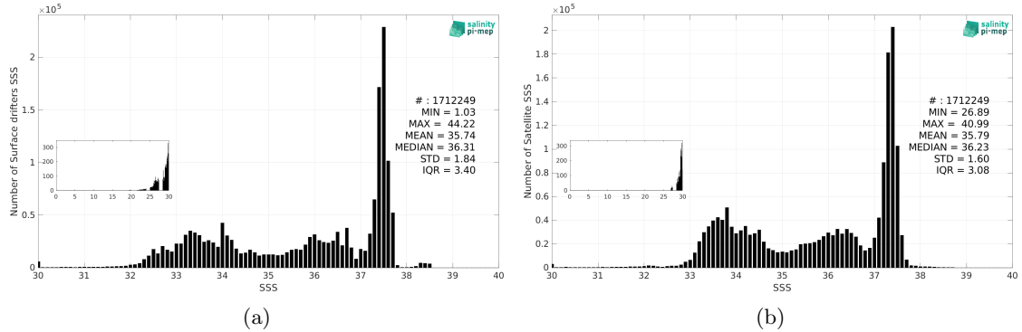
Figure 3: Histograms of SSS from Surface drifters (a) and SMOS SSS L4 v2 - Daily (BEC) (b) considering all match-up pairs per bins of 0.1 over the Mid-Low Latitudes 45N-45S Pi-MEP region and for the full satellite product period.
