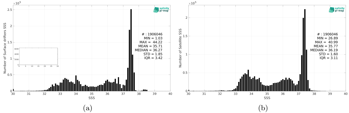
Figure 2: Histograms of SSS from Surface drifters (a) and SMOS SSS L4 v2 - Daily (BEC) (b) considering all match-up pairs per bins of 0.1 over the Mid-Low Latitudes 45N-45S Pi-MEP region and for the full satellite product period.
