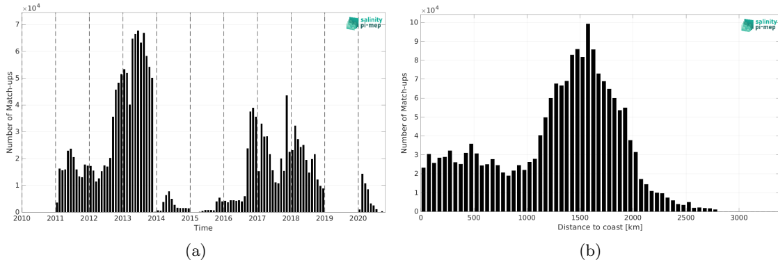
Figure 1: Number of match-ups between Surface drifters and SMOS SSS L4 v2 - Daily (BEC) SSS as a function of time (a) and as function of the distance to coast (b) over the Mid-Low Latitudes 45N-45S Pi-MEP region and for the full satellite product period.
