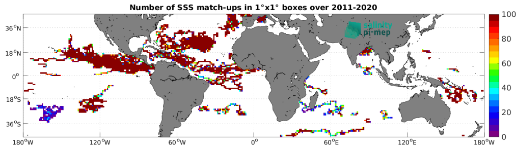
Figure 3: Number of SSS match-ups between Surface drifters SSS and the SMOS SSS L4 v2 - Daily (BEC) SSS product for the Mid-Low Latitudes 45N-45S Pi-MEP region over 1^\circ \times 1^\circ boxes and for the full satellite product period.
