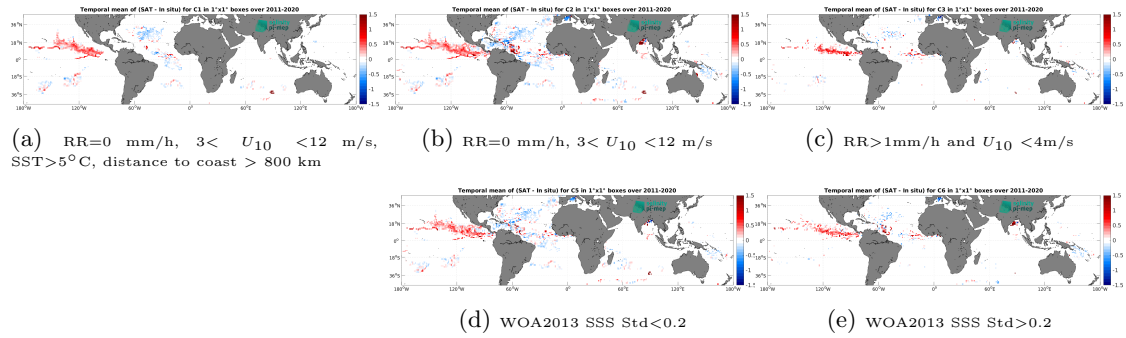
Figure 11: Temporal mean gridded over spatial boxes of size 1^\circ \times 1^\circ of \Delta SSS (SMOS SSS L4 v2 - Daily (BEC) - Surface drifters) for 5 different subdatasets corresponding to:RR=0 mm/h, 3 < U_{10} < 12 m/s, SST >5^\circ\text{C} , distance to coast > 800 km (a), RR=0 mm/h, 3 < U_{10} < 12 m/s (b), RR >1 mm/h and U_{10} < 4 m/s (c), WOA2013 SSS Std <0.2 (d), WOA2013 SSS Std >0.2 (e).
