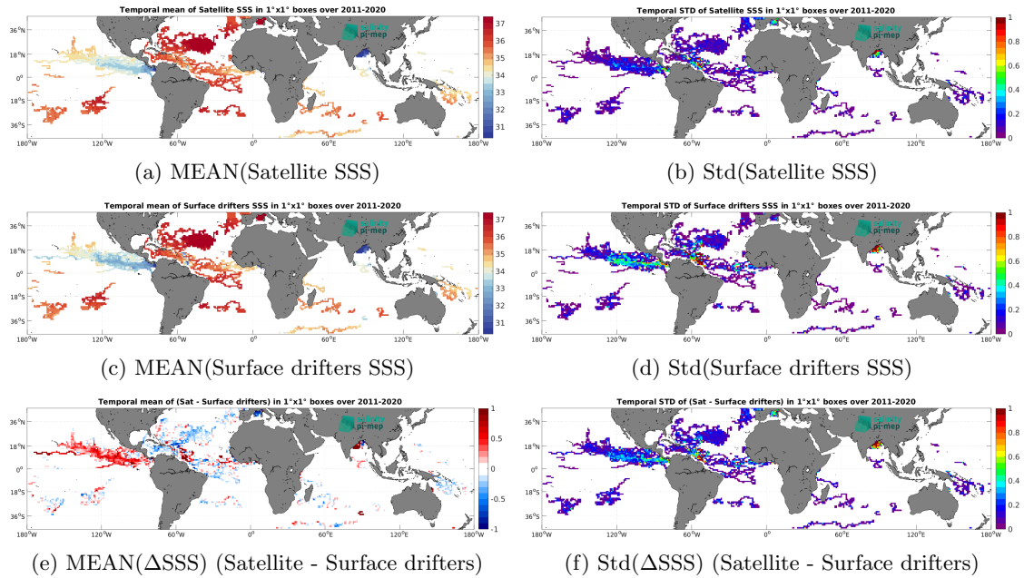
Figure 5: Temporal mean (left) and Std (right) of SSS from SMOS SSS L4 v2 - Daily (BEC) (top), Surface drifters (middle), and of \Delta SSS (Satellite - Surface drifters). Only match-up pairs are used to generate these maps.
