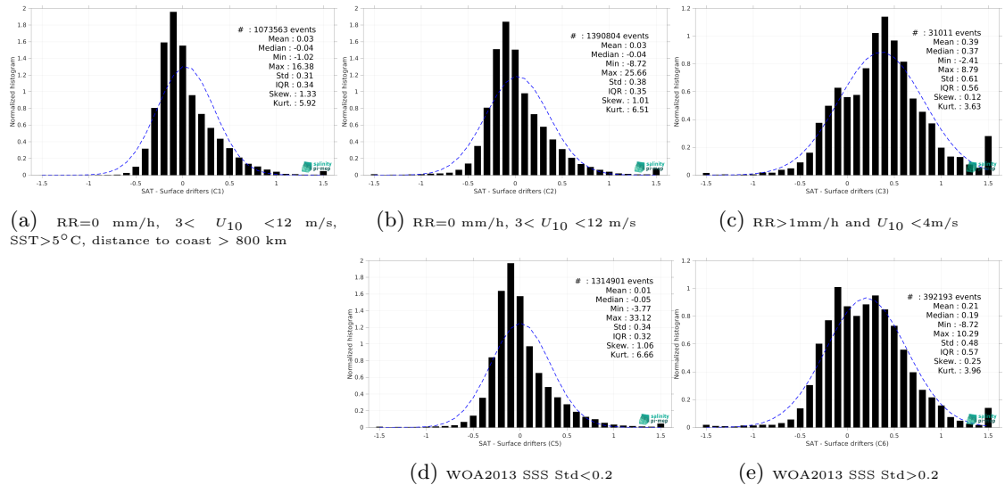
Figure 12: Normalized histogram of \Delta SSS (SMOS SSS L4 v2 - Daily (BEC) - Surface drifters) for 5 different subdatasets corresponding to: RR=0 mm/h, 3 < U_{10} < 12 m/s, SST >5^\circ\text{C} , distance to coast > 800 km (a), RR=0 mm/h, 3 < U_{10} < 12 m/s (b), RR >1 mm/h and U_{10} < 4 m/s (c), WOA2013 SSS Std <0.2 (d), WOA2013 SSS Std >0.2 (e).
