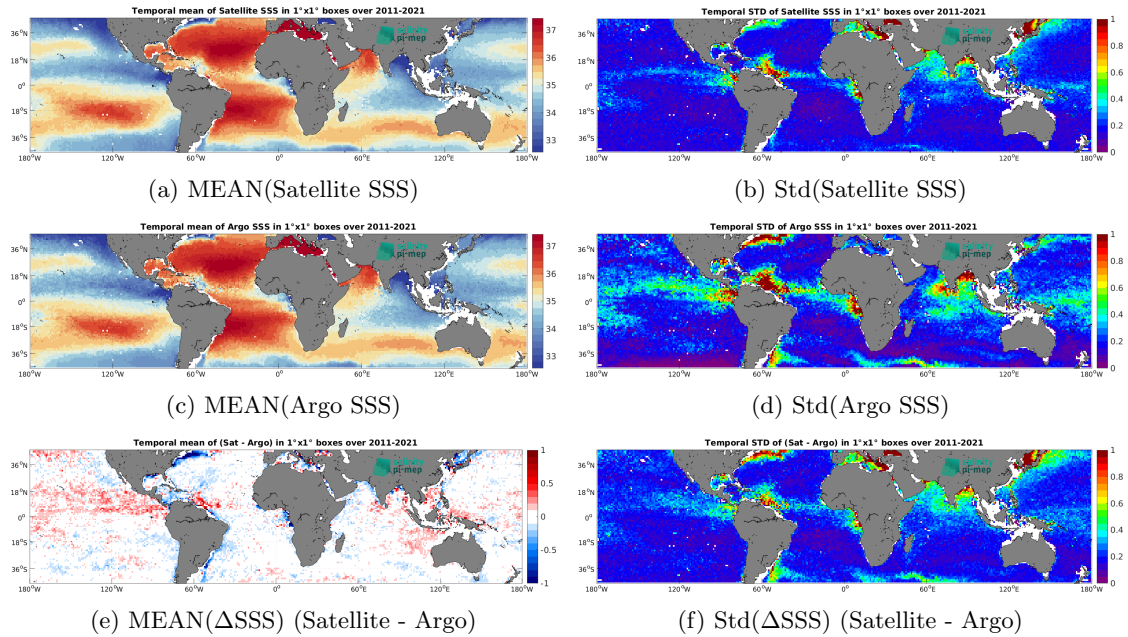
Figure 7: Temporal mean (left) and Std (right) of SSS from SMOS SSS L4 v2 - Daily (BEC) (top), Argo (middle), and of \Delta SSS (Satellite - Argo). Only match-up pairs are used to generate these maps.
