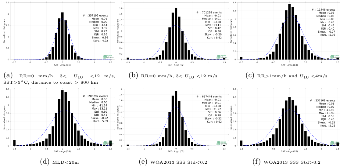
Figure 13: Normalized histogram of \Delta SSS (SMOS SSS L4 v2 - Daily (BEC) - Argo) for 6 different subdatasets corresponding to: RR=0 mm/h, 3 < U_{10} < 12 m/s, SST > 5°C, distance to coast > 800 km (a), RR=0 mm/h, 3 < U_{10} < 12 m/s (b), RR > 1mm/h and U_{10} < 4 m/s (c), MLD < 20m (d), WOA2013 SSS Std < 0.2 (e), WOA2013 SSS Std > 0.2 (f).
