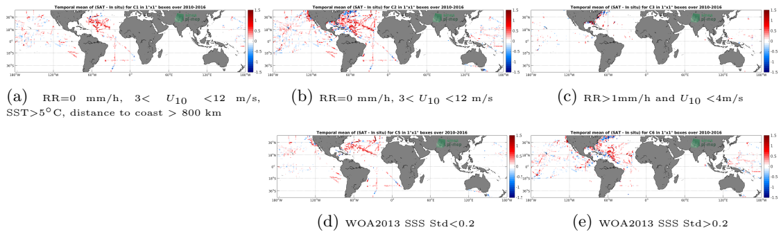
Figure 12: Temporal mean gridded over spatial boxes of size 1^\circ \times 1^\circ of \Delta SSS (SMOS SSS L3 v3 Monthly (ICDC) - TSG (SAMOS)) for 5 different subdatasets corresponding to: RR=0 mm/h, 3 < U_{10} < 12 m/s, SST > 5^\circ C , distance to coast > 800 km (a), RR=0 mm/h, 3 < U_{10} < 12 m/s (b), RR>1mm/h and U_{10} < 4 m/s (c), WOA2013 SSS Std<0.2 (d), WOA2013 SSS Std>0.2 (e).
