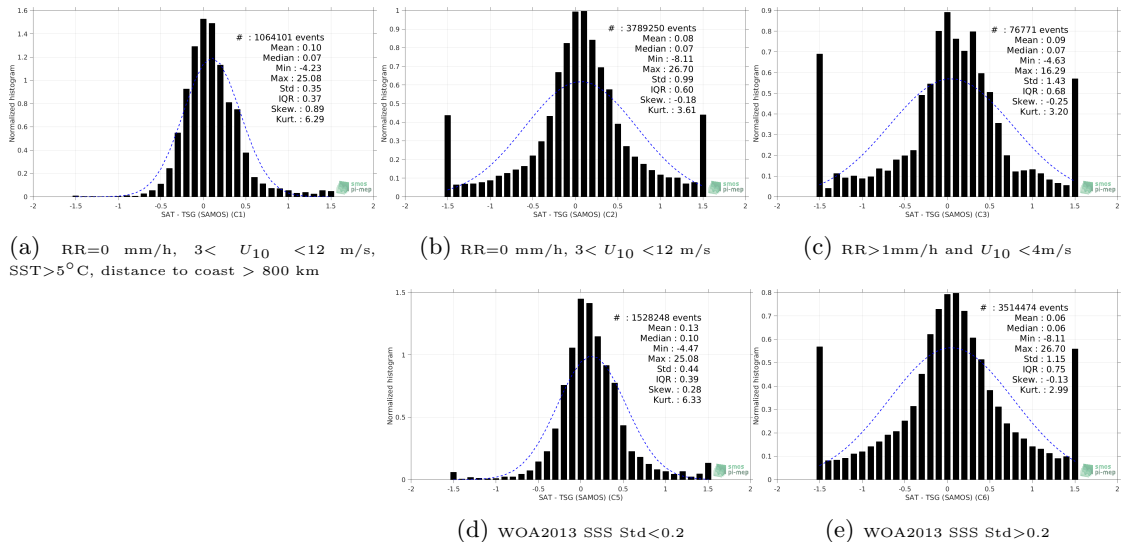
Figure 13: Normalized histogram of \Delta SSS (SMOS SSS L3 v3 Monthly (ICDC) - TSG (SAMOS)) for 5 different subdatasets corresponding to: RR=0 mm/h, 3 < U_{10} < 12 m/s, SST > 5^\circ C , distance to coast > 800 km (a), RR=0 mm/h, 3 < U_{10} < 12 m/s (b), RR>1mm/h and U_{10} < 4 m/s (c), WOA2013 SSS Std<0.2 (d), WOA2013 SSS Std>0.2 (e).
