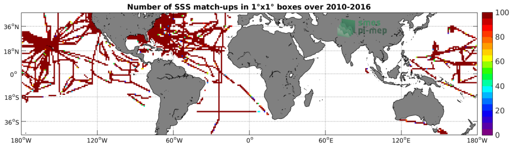
Figure 4: Number of SSS match-ups between TSG (SAMOS) SSS and the SMOS SSS L3 v3 Monthly (ICDC) SSS product for the Mid-Low Latitudes 45N-45S Pi-MEP region over 1^\circ \times 1^\circ boxes and for the full satellite product period.
