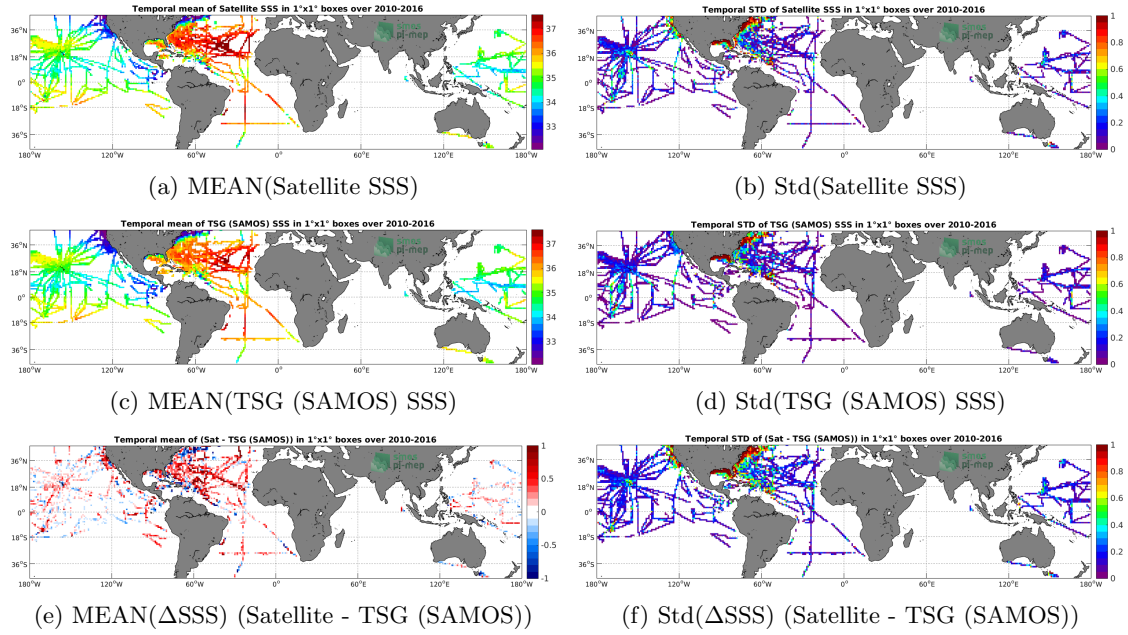
Figure 6: Temporal mean (left) and Std (right) of SSS from SMOS SSS L3 v3 Monthly (ICDC) (top), TSG (SAMOS) (middle), and of \Delta SSS (Satellite - TSG (SAMOS)). Only match-up pairs are used to generate these maps.
