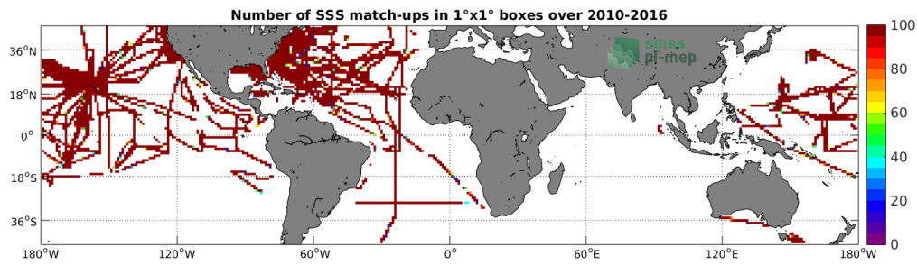
Figure 4: Number of SSS match-ups between TSG-SAMOS SSS and the SMOS-L3-ICDC-V3-MONTHLY-0.5DEG SSS product for the Mid-Low Latitudes 45N-45S Pi-MEP region over 1^\circ \times 1^\circ boxes and for the full satellite product period.
