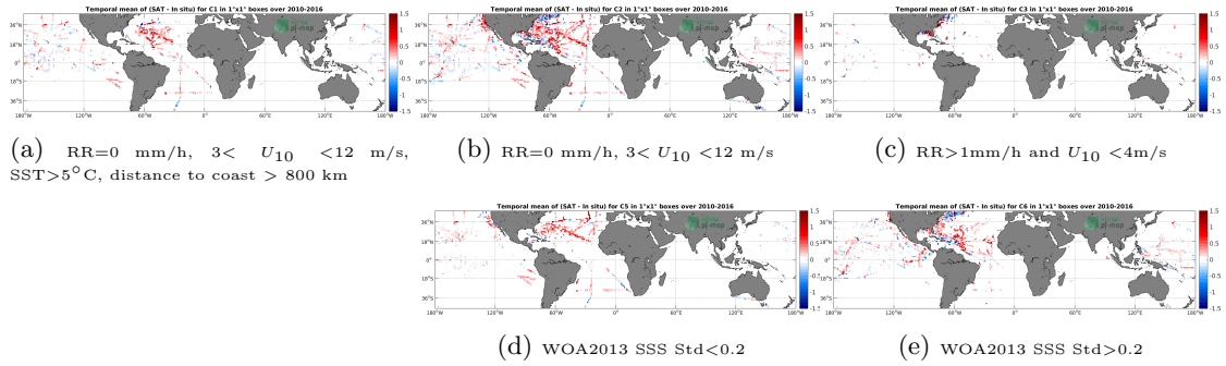
Figure 12: Temporal mean gridded over spatial boxes of size 1°x1° of \Delta SSS (SMOS-L3-ICDC-V3-MONTHLY-0.5DEG - TSG-SAMOS) for 5 different subdatasets corresponding to: RR=0 mm/h, 3 < U_{10} < 12 m/s, SST > 5°C, distance to coast > 800 km (a), RR=0 mm/h, 3 < U_{10} < 12 m/s (b), RR > 1mm/h and U_{10} < 4m/s (c), WOA2013 SSS Std < 0.2 (d), WOA2013 SSS Std > 0.2 (e).
