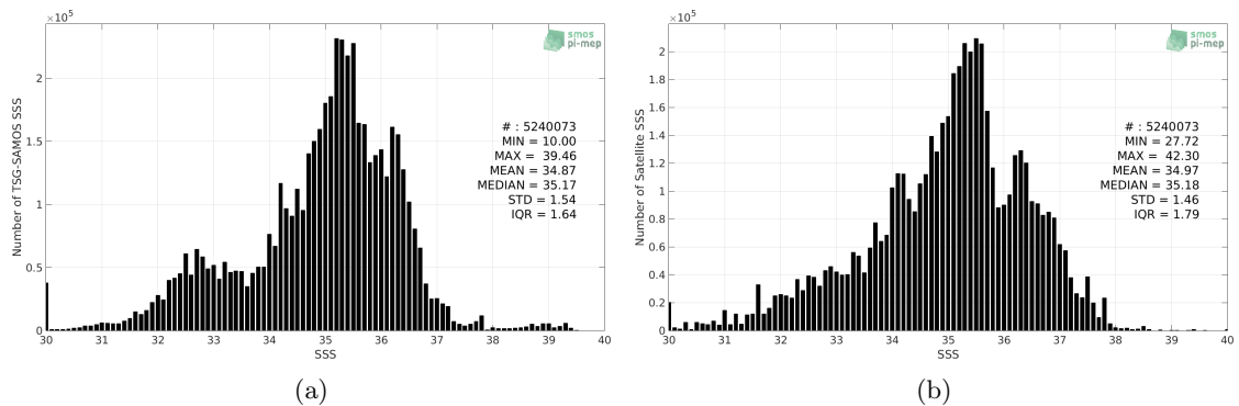
Figure 2: Histograms of SSS from TSG-SAMOS (a) and SMOS-L3-ICDC-V3-MONTHLY-0.5DEG (b) considering all match-up pairs per bins of 0.1 over the Mid-Low Latitudes 45N-45S Pi-MEP region and for the full satellite product period.
