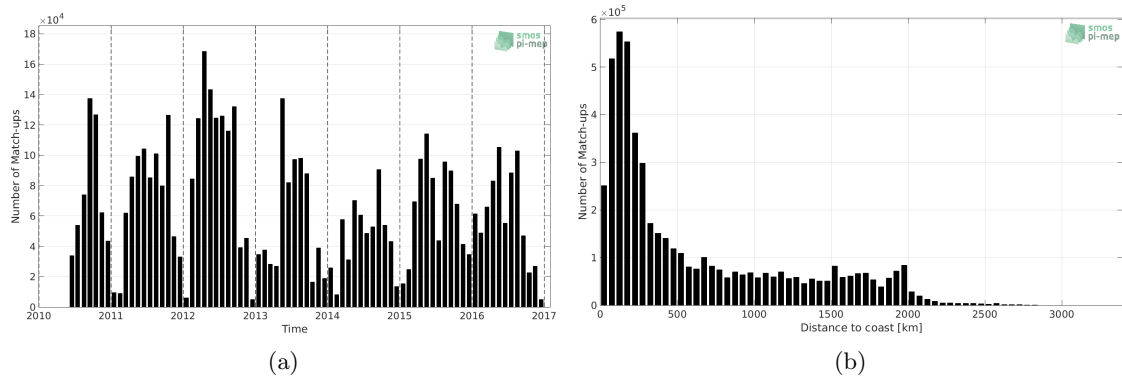
Figure 1: Number of match-ups between TSG-SAMOS and SMOS-L3-ICDC-V3-MONTHLY-0.5DEG SSS as a function of time (a) and as function of the distance to coast (b) over the Mid-Low Latitudes 45N-45S Pi-MEP region and for the full satellite product period.
