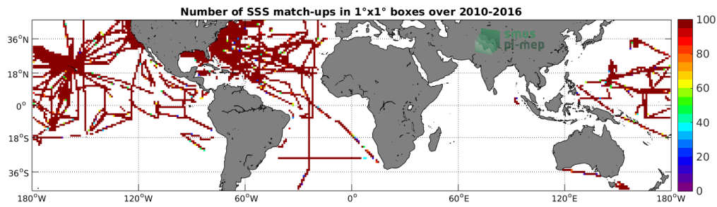
Figure 4: Number of SSS match-ups between TSG-SAMOS SSS and the SMOS-L3-ICDC-V3-MONTHLY-0.5DEG SSS product for the Mid-Low Latitudes 45N-45S Pi-MEP region over 1°x1° boxes and for the full satellite product period.
