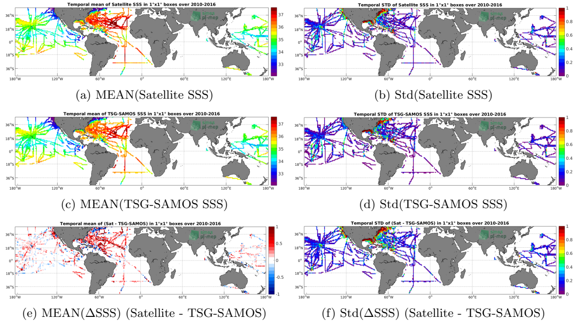
Figure 6: Temporal mean (left) and Std (right) of SSS from SMOS-L3-ICDC-V3-MONTHLY-0.5DEG (top), TSG-SAMOS (middle), and of \Delta SSS (Satellite - TSG-SAMOS). Only match-up pairs are used to generate these maps.
