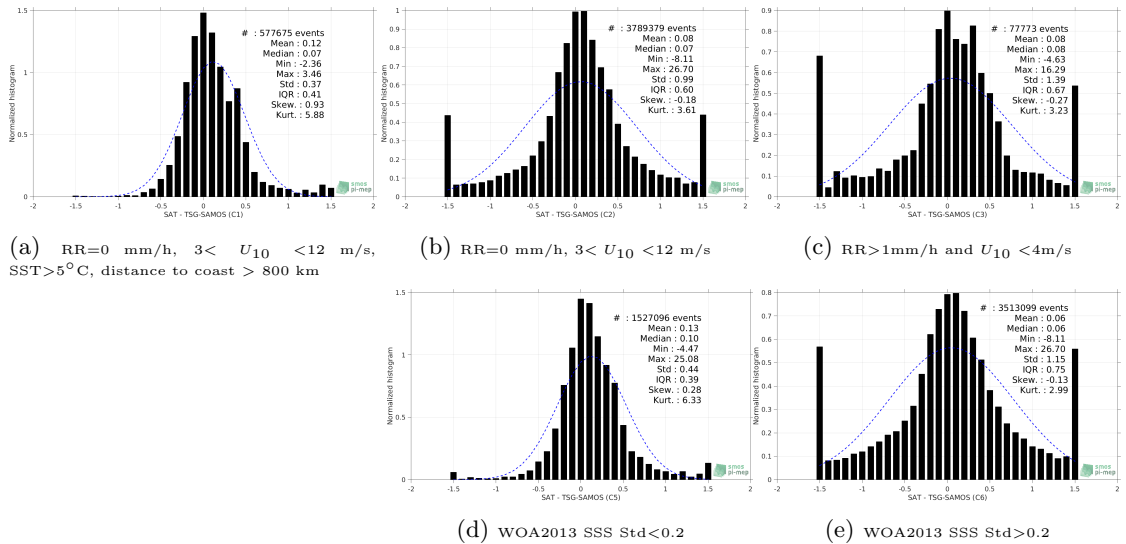
Figure 13: Normalized histogram of \Delta SSS (SMOS-L3-ICDC-V3-MONTHLY-0.5DEG - TSG-SAMOS) for 5 different subdatasets corresponding to: RR=0 mm/h, 3 < U_{10} < 12 m/s, SST >5^\circ C, distance to coast > 800 km (a), RR=0 mm/h, 3 < U_{10} < 12 m/s (b), RR >1 mm/h and U_{10} < 4 m/s (c), WOA2013 SSS Std <0.2 (d), WOA2013 SSS Std >0.2 (e).
