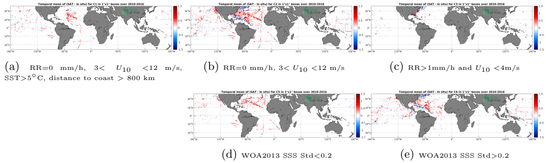
Figure 12: Temporal mean gridded over spatial boxes of size 1^\circ \times 1^\circ of \Delta SSS (SMOS-L3-ICDC-V3-MONTHLY-0.5DEG - TSG-SAMOS) for 5 different subdatasets corresponding to: RR=0 mm/h, 3 < U_{10} < 12 m/s, SST >5^\circ C, distance to coast > 800 km (a), RR=0 mm/h, 3 < U_{10} < 12 m/s (b), RR >1 mm/h and U_{10} < 4 m/s (c), WOA2013 SSS Std <0.2 (d), WOA2013 SSS Std >0.2 (e).
