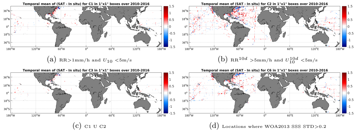
Figure 12: Temporal mean gridded over spatial boxes of size 1^\circ \times 1^\circ of \Delta SSS (SMOS-L3-ICDC-V3-MONTHLY-0.5DEG - TSG-SAMOS) for 4 different subdatasets corresponding to: RR > 1\text{mm/h} and U_{10} < 5\text{m/s} (a), RR^{10d} > 5\text{mm/h} and U_{10}^{10d} < 5\text{m/s} (b), C1 U C2 (c), Locations where WOA2013 SSS STD > 0.2 (d).
