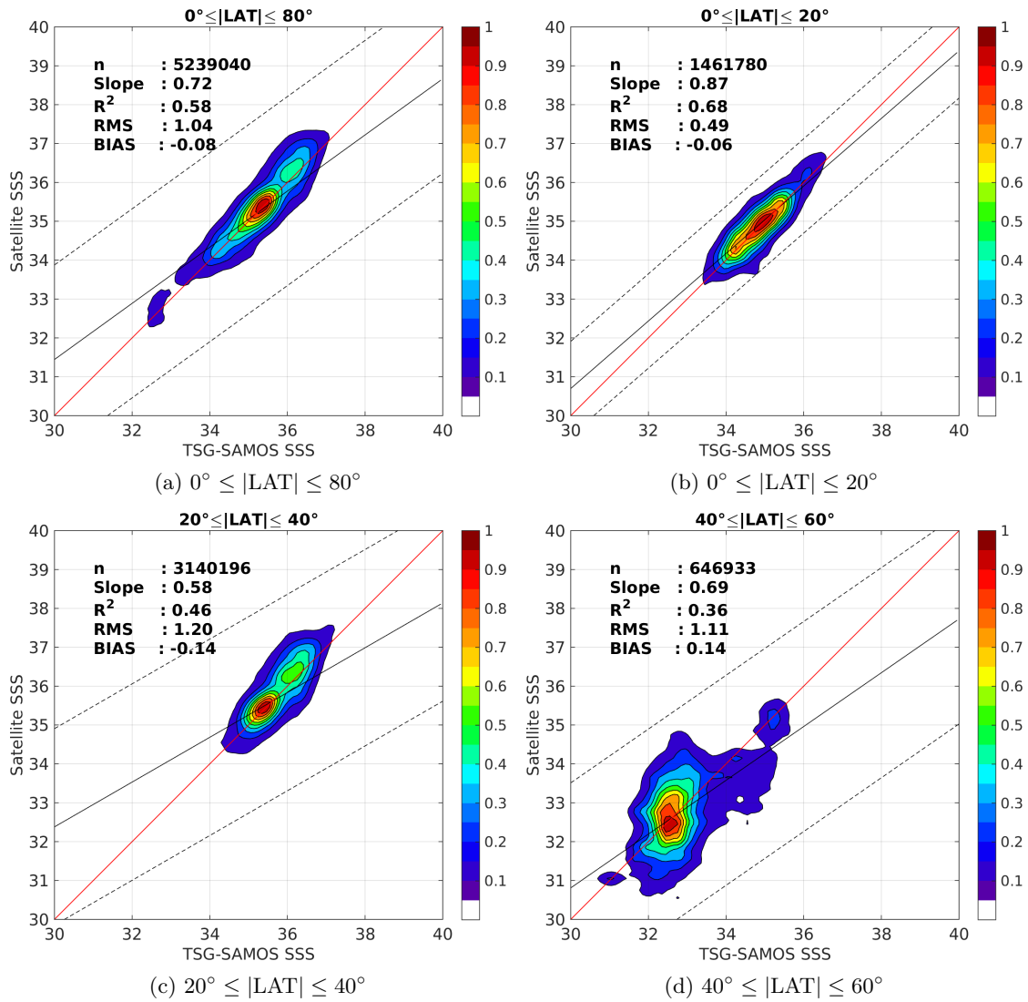
Figure 9: Contour maps of the concentration of SMOS-L3-ICDC-V3-MONTHLY-0.5DEG SSS (y-axis) versus TSG-SAMOS SSS (x-axis) at match-up pairs for different latitude bands. For each plot, the red line shows x=y . The black thin and dashed lines indicate a linear fit through the data cloud and the \pm 95\% confidence levels, respectively. The number match-up pairs n , the slope and R^2 coefficient of the linear fit, the root mean square (RMS) and the mean bias between satellite and in situ data are indicated for each latitude band in each plots.
