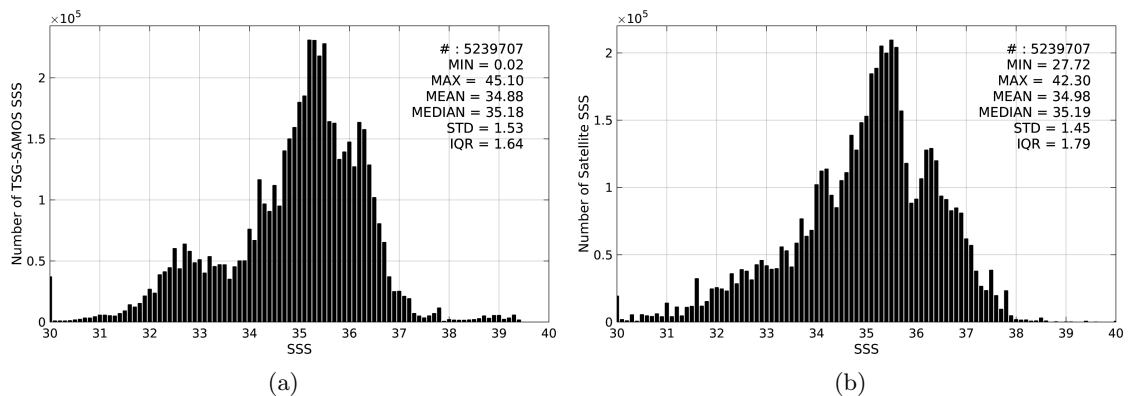
Figure 2: Histograms of SSS from TSG-SAMOS (a) and SMOS-L3-ICDC-V3-MONTHLY-0.5DEG (b) considering all match-up pairs per bins of 0.1 over the Mid-Low Latitudes 45N-45S Pi-MEP region and for the full satellite product period.
