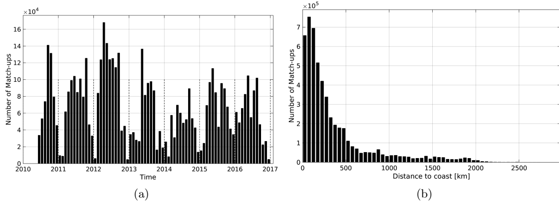
Figure 1: Number of match-ups between TSG-SAMOS and SMOS-L3-ICDC-V3-MONTHLY-0.5DEG SSS as a function of time (a) and as function of the distance to coast (b) over the Mid-Low Latitudes 45N-45S Pi-MEP region and for the full satellite product period.
