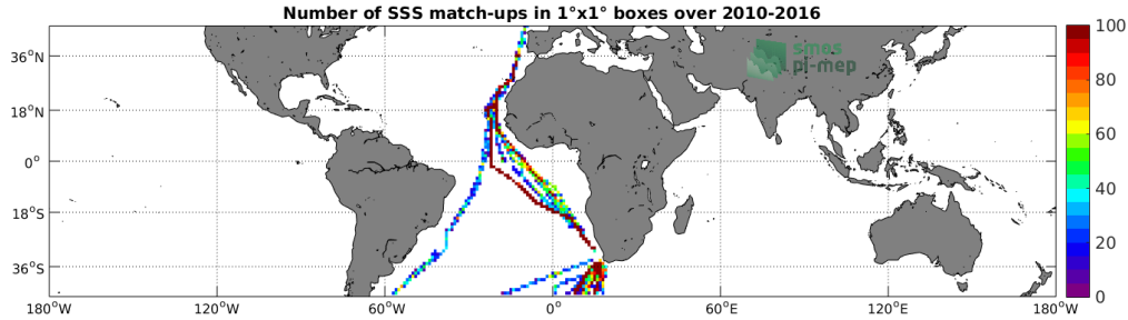
Figure 4: Number of SSS match-ups between TSG-POLARSTERN SSS and the SMOS-L3-ICDC-V3-MONTHLY-0.5DEG SSS product for the Mid-Low Latitudes 45N-45S Pi-MEP region over 1°x1° boxes and for the full satellite product period.
