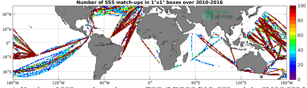
Figure 4: Number of SSS match-ups between TSG (LEGOS-DM) SSS and the SMOS SSS L3 v3 Monthly (ICDC) SSS product for the Mid-Low Latitudes 45N-45S Pi-MEP region over 1^\circ \times 1^\circ boxes and for the full satellite product period.
