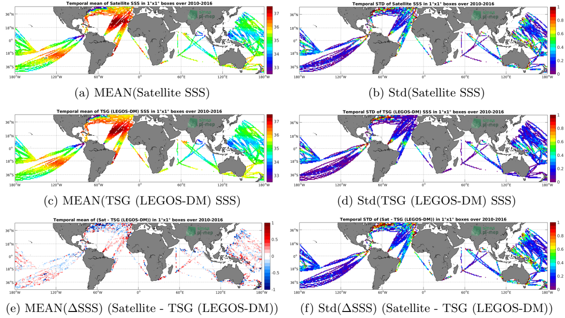
Figure 6: Temporal mean (left) and Std (right) of SSS from SMOS SSS L3 v3 Monthly (ICDC) (top), TSG (LEGOS-DM) (middle), and of \Delta SSS (Satellite - TSG (LEGOS-DM)). Only match-up pairs are used to generate these maps.
