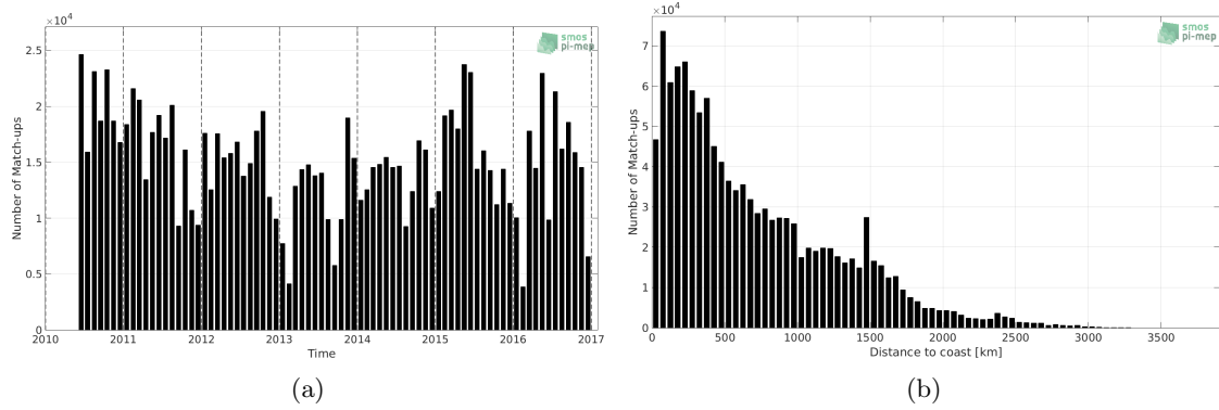
Figure 1: Number of match-ups between TSG (LEGOS-DM) and SMOS SSS L3 v3 Monthly (ICDC) SSS as a function of time (a) and as function of the distance to coast (b) over the Mid-Low Latitudes 45N-45S Pi-MEP region and for the full satellite product period.
