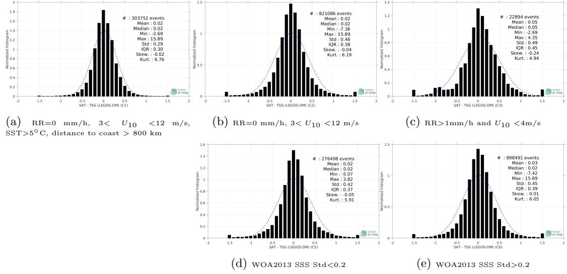
Figure 13: Normalized histogram of \Delta\text{SSS} (SMOS SSS L3 v3 Monthly (ICDC) - TSG (LEGOS-DM)) for 5 different subdatasets corresponding to: RR=0 mm/h, 3 < U_{10} < 12 m/s, SST>5°C, distance to coast > 800 km (a), RR=0 mm/h, 3 < U_{10} < 12 m/s (b), RR>1mm/h and U_{10} < 4 m/s (c), WOA2013 SSS Std<0.2 (d), WOA2013 SSS Std>0.2 (e).
