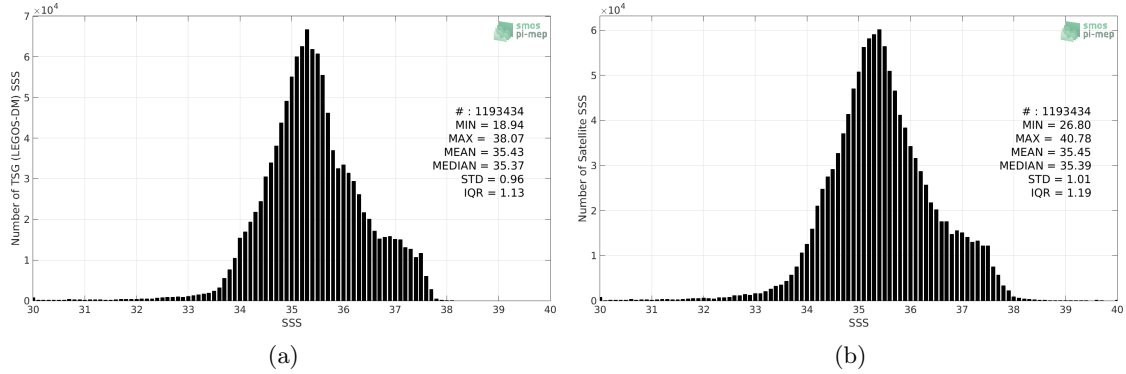
Figure 2: Histograms of SSS from TSG (LEGOS-DM) (a) and SMOS SSS L3 v3 Monthly (ICDC) (b) considering all match-up pairs per bins of 0.1 over the Mid-Low Latitudes 45N-45S Pi-MEP region and for the full satellite product period.
