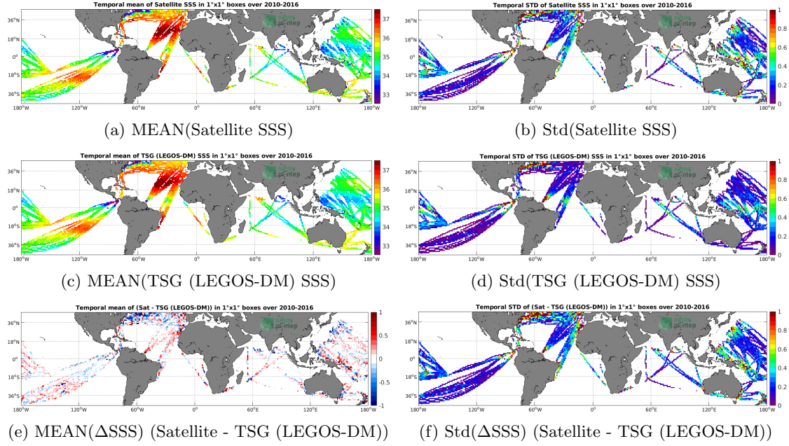
Figure 6: Temporal mean (left) and Std (right) of SSS from SMOS SSS L3 v3 Monthly (ICDC) (top), TSG (LEGOS-DM) (middle), and of \Delta SSS (Satellite - TSG (LEGOS-DM)). Only match-up pairs are used to generate these maps.
