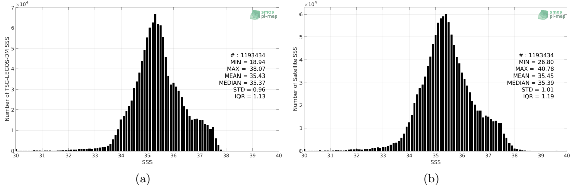
Figure 2: Histograms of SSS from TSG-LEGOS-DM (a) and SMOS-L3-ICDC-V3-MONTHLY-0.5DEG (b) considering all match-up pairs per bins of 0.1 over the Mid-Low Latitudes 45N-45S Pi-MEP region and for the full satellite product period.
