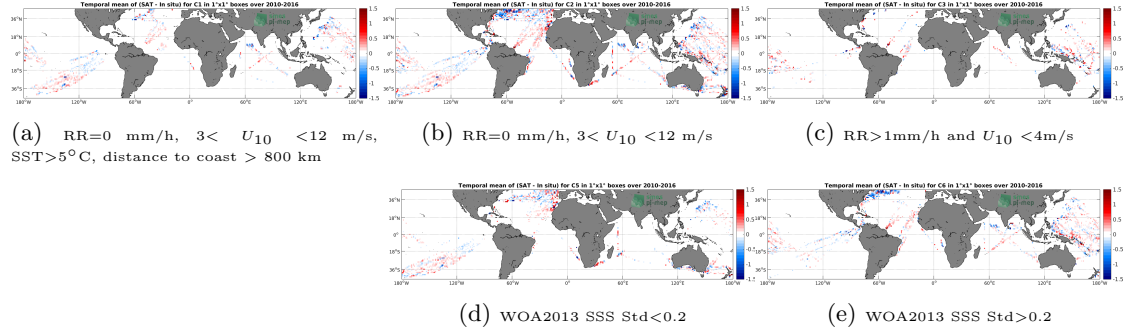
Figure 12: Temporal mean gridded over spatial boxes of size 1^\circ \times 1^\circ of \Delta SSS (SMOS-L3-ICDC-V3-MONTHLY-0.5DEG - TSG-LEGOS-DM) for 5 different subdatasets corresponding to: RR=0 mm/h, 3 < U_{10} < 12 m/s, SST > 5^\circ C , distance to coast > 800 km (a), RR=0 mm/h, 3 < U_{10} < 12 m/s (b), RR > 1 mm/h and U_{10} < 4 m/s (c), WOA2013 SSS Std < 0.2 (d), WOA2013 SSS Std > 0.2 (e).
