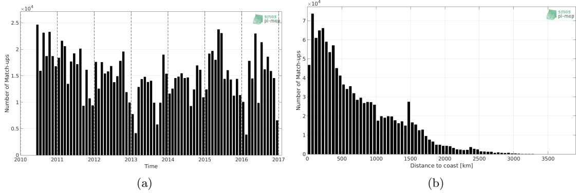
Figure 1: Number of match-ups between TSG-LEGOS-DM and SMOS-L3-ICDC-V3-MONTHLY-0.5DEG SSS as a function of time (a) and as function of the distance to coast (b) over the Mid-Low Latitudes 45N-45S Pi-MEP region and for the full satellite product period.
