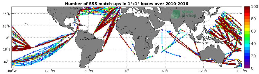
Figure 4: Number of SSS match-ups between TSG-LEGOS-DM SSS and the SMOS-L3-ICDC-V3-MONTHLY-0.5DEG SSS product for the Mid-Low Latitudes 45N-45S Pi-MEP region over 1^\circ \times 1^\circ boxes and for the full satellite product period.
