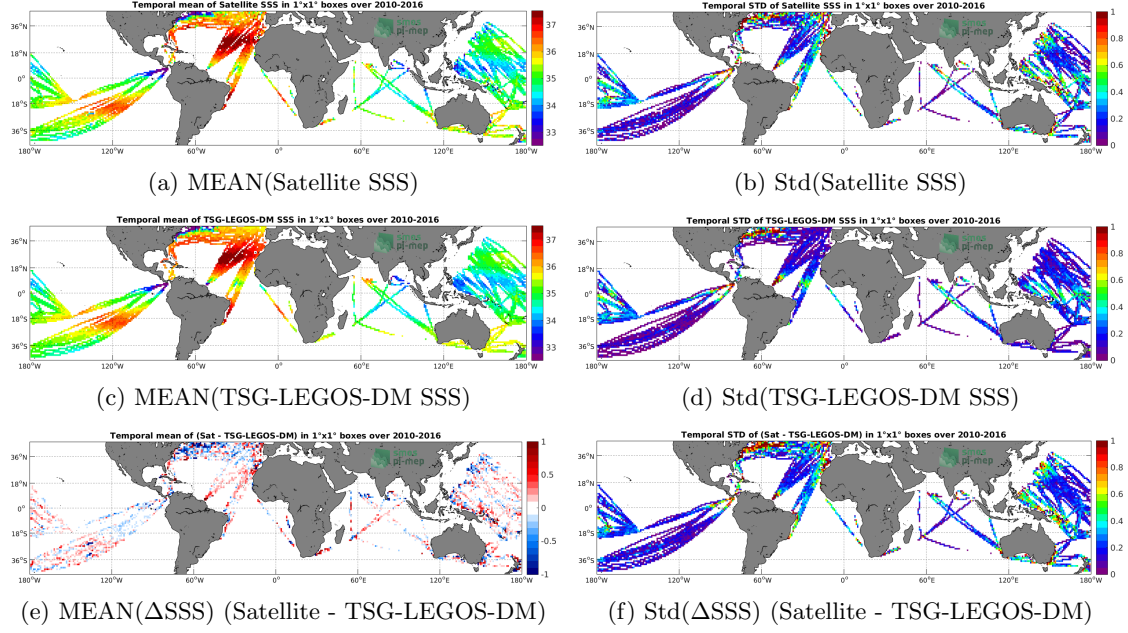
Figure 6: Temporal mean (left) and Std (right) of SSS from SMOS-L3-ICDC-V3-MONTHLY-0.5DEG (top), TSG-LEGOS-DM (middle), and of \Delta SSS (Satellite - TSG-LEGOS-DM). Only match-up pairs are used to generate these maps.
