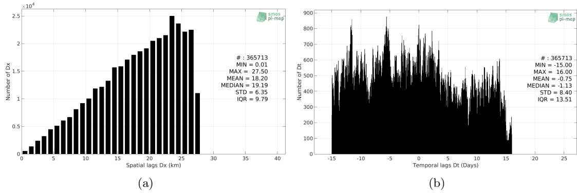
Figure 5: Histograms of the spatial (a) and temporal (b) lags between the location/time of the TSG (GOSUD-Sailing-ship) measurement and the date of the corresponding SMOS SSS L3 v3 Monthly (ICDC) SSS pixel.
