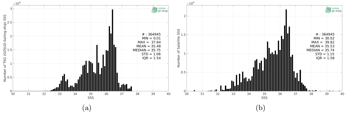
Figure 2: Histograms of SSS from TSG (GOSUD-Sailing-ship) (a) and SMOS SSS L3 v3 Monthly (ICDC) (b) considering all match-up pairs per bins of 0.1 over the Mid-Low Latitudes 45N-45S Pi-MEP region and for the full satellite product period.
