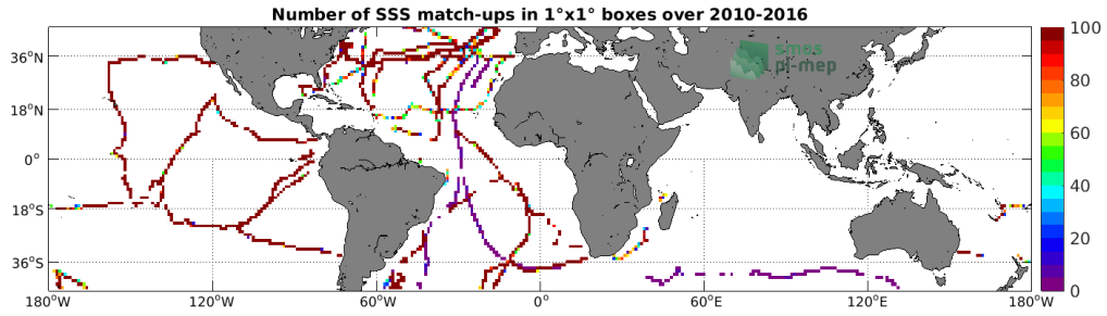
Figure 4: Number of SSS match-ups between TSG (GOSUD-Sailing-ship) SSS and the SMOS SSS L3 v3 Monthly (ICDC) SSS product for the Mid-Low Latitudes 45N-45S Pi-MEP region over 1^\circ \times 1^\circ boxes and for the full satellite product period.
