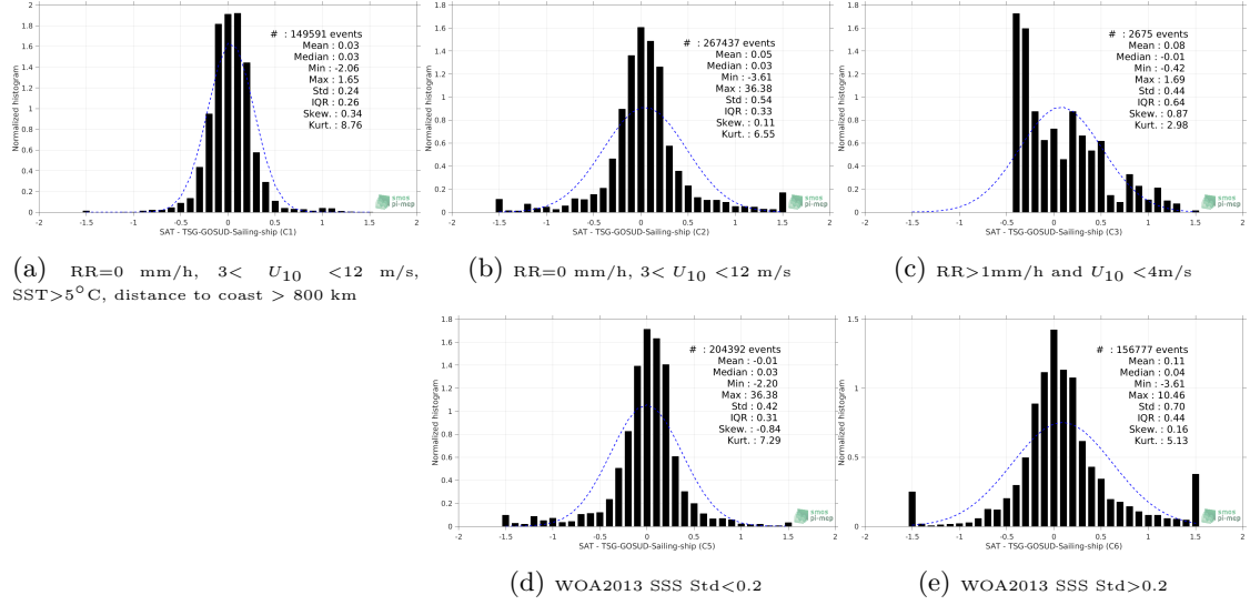
Figure 13: Normalized histogram of \Delta SSS (SMOS-L3-ICDC-V3-MONTHLY-0.5DEG - TSG-GOSUD-Sailing-ship) for 5 different subdatasets corresponding to: RR=0 mm/h, 3 < U_{10} < 12 m/s, SST>5°C, distance to coast > 800 km (a), RR=0 mm/h, 3 < U_{10} < 12 m/s (b), RR>1 mm/h and U_{10} < 4 m/s (c), WOA2013 SSS Std<0.2 (d), WOA2013 SSS Std>0.2 (e).
