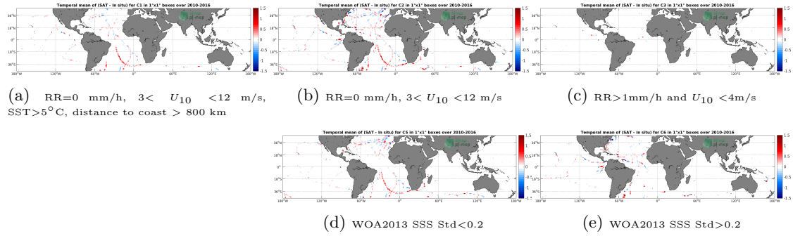
Figure 12: Temporal mean gridded over spatial boxes of size 1^\circ \times 1^\circ of \Delta SSS (SMOS-L3-ICDC-V3-MONTHLY-0.5DEG - TSG-GOSUD-Sailing-ship) for 5 different subdatasets corresponding to: RR=0 mm/h, 3 < U_{10} < 12 m/s, SST > 5^\circ C , distance to coast > 800 km (a), RR=0 mm/h, 3 < U_{10} < 12 m/s (b), RR > 1 mm/h and U_{10} < 4 m/s (c), WOA2013 SSS Std < 0.2 (d), WOA2013 SSS Std > 0.2 (e).
