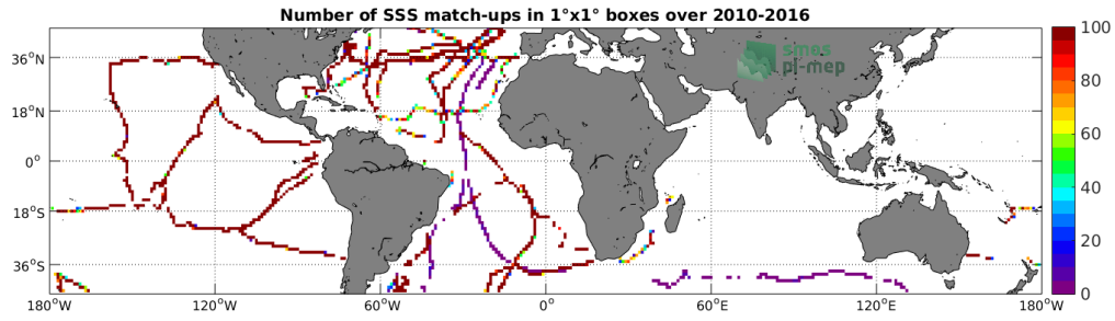
Figure 4: Number of SSS match-ups between TSG-GOSUD-Sailing-ship SSS and the SMOS-L3-ICDC-V3-MONTHLY-0.5DEG SSS product for the Mid-Low Latitudes 45N-45S Pi-MEP region over 1°x1° boxes and for the full satellite product period.
