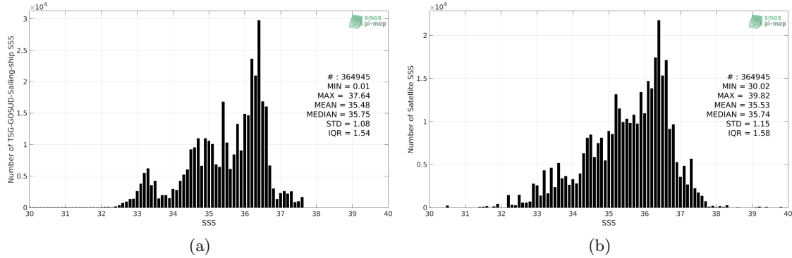
Figure 2: Histograms of SSS from TSG-GOSUD-Sailing-ship (a) and SMOS-L3-ICDC-V3-MONTHLY-0.5DEG (b) considering all match-up pairs per bins of 0.1 over the Mid-Low Latitudes 45N-45S Pi-MEP region and for the full satellite product period.
