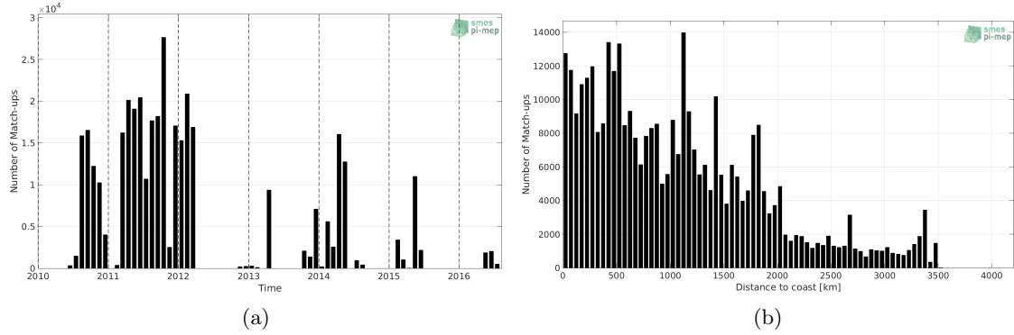
Figure 1: Number of match-ups between TSG-GOSUD-Sailing-ship and SMOS-L3-ICDC-V3-MONTHLY-0.5DEG SSS as a function of time (a) and as function of the distance to coast (b) over the Mid-Low Latitudes 45N-45S Pi-MEP region and for the full satellite product period.
