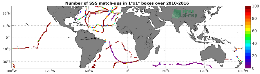
Figure 4: Number of SSS match-ups between TSG-GOSUD-Sailing-ship SSS and the SMOS-L3-ICDC-V3-MONTHLY-0.5DEG SSS product for the Mid-Low Latitudes 45N-45S Pi-MEP region over 1^\circ \times 1^\circ boxes and for the full satellite product period.
