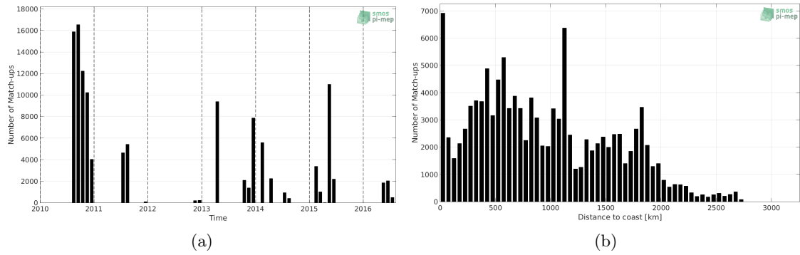
Figure 1: Number of match-ups between TSG-GOSUD-Sailing-ship and SMOS-L3-ICDC-V3-MONTHLY-0.5DEG SSS as a function of time (a) and as function of the distance to coast (b) over the Mid-Low Latitudes 45N-45S Pi-MEP region and for the full satellite product period.
