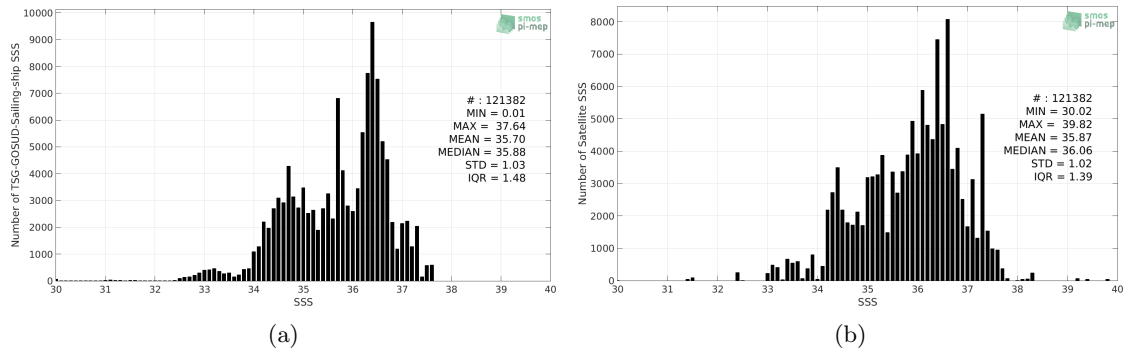
Figure 2: Histograms of SSS from TSG-GOSUD-Sailing-ship (a) and SMOS-L3-ICDC-V3-MONTHLY-0.5DEG (b) considering all match-up pairs per bins of 0.1 over the Mid-Low Latitudes 45N-45S Pi-MEP region and for the full satellite product period.
