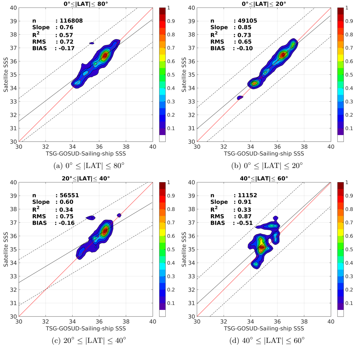
Figure 9: Contour maps of the concentration of SMOS-L3-ICDC-V3-MONTHLY-0.5DEG SSS (y-axis) versus TSG-GOSUD-Sailing-ship SSS (x-axis) at match-up pairs for different latitude bands. For each plot, the red line shows x=y . The black thin and dashed lines indicate a linear fit through the data cloud and the \pm 95\% confidence levels, respectively. The number match-up pairs n , the slope and R^2 coefficient of the linear fit, the root mean square (RMS) and the mean bias between satellite and in situ data are indicated for each latitude band in each plots.
