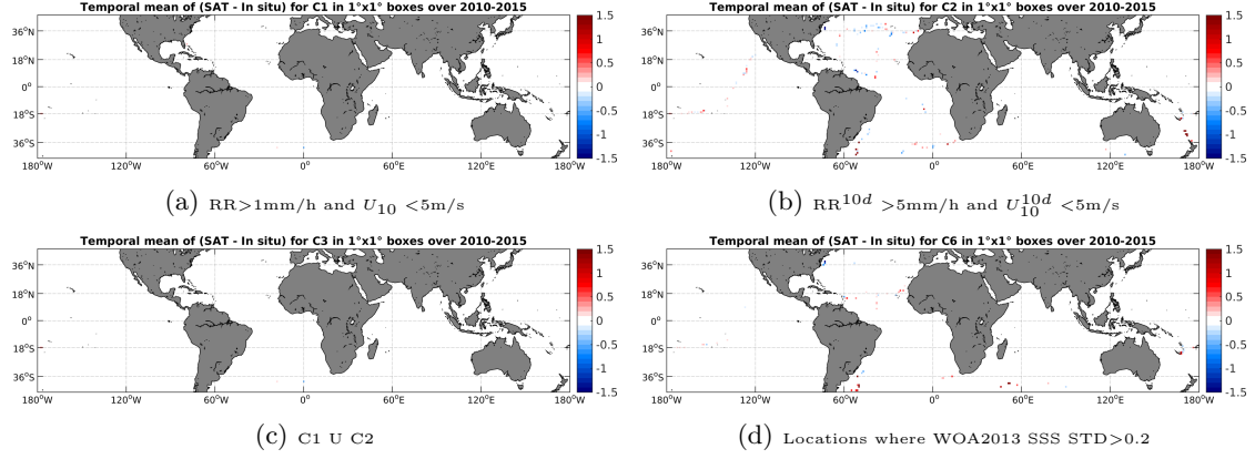
Figure 12: Temporal mean gridded over spatial boxes of size 1^\circ \times 1^\circ of \Delta SSS (SMOS-L3-ICDC-V3-MONTHLY-0.5DEG - TSG-GOSUD-Sailing-ship) for 4 different subdatasets corresponding to: RR > 1 mm/h and U_{10} < 5 m/s (a), RR^{10d} > 5 mm/h and U_{10}^{10d} < 5 m/s (b), C1 U C2 (c), Locations where WOA2013 SSS STD > 0.2 (d).
