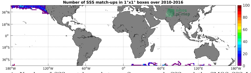
Figure 4: Number of SSS match-ups between Sea mammals SSS and the SMOS SSS L3 v3 Monthly (ICDC) SSS product for the Mid-Low Latitudes 45N-45S Pi-MEP region over 1^\circ \times 1^\circ boxes and for the full satellite product period.
