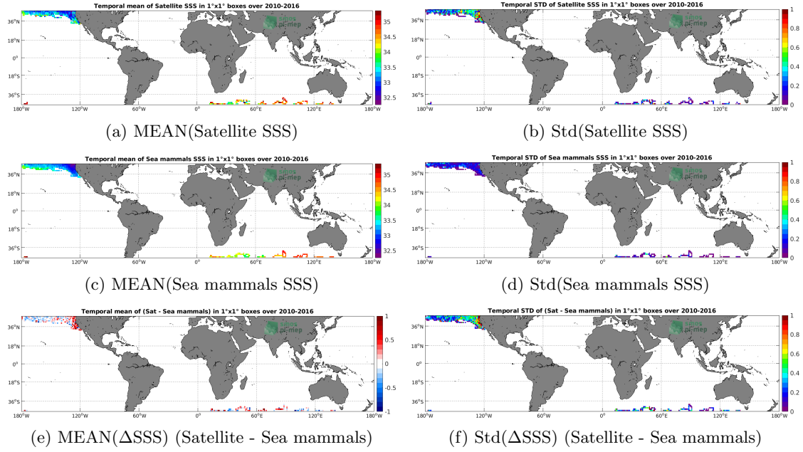
Figure 6: Temporal mean (left) and Std (right) of SSS from SMOS SSS L3 v3 Monthly (ICDC) (top), Sea mammals (middle), and of \Delta SSS (Satellite - Sea mammals). Only match-up pairs are used to generate these maps.
