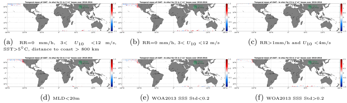
Figure 12: Temporal mean gridded over spatial boxes of size 1^\circ \times 1^\circ of \Delta SSS (SMOS SSS L3 v3 Monthly (ICDC) - Sea mammals) for 6 different subdatasets corresponding to: RR=0 mm/h, 3 < U_{10} < 12 m/s, SST > 5^\circ C , distance to coast > 800 km (a), RR=0 mm/h, 3 < U_{10} < 12 m/s (b), RR > 1 mm/h and U_{10} < 4 m/s (c), MLD < 20 m (d), WOA2013 SSS Std < 0.2 (e), WOA2013 SSS Std > 0.2 (f).
