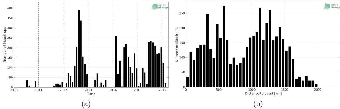
Figure 1: Number of match-ups between Sea mammals and SMOS SSS L3 v3 Monthly (ICDC) SSS as a function of time (a) and as function of the distance to coast (b) over the Mid-Low Latitudes 45N-45S Pi-MEP region and for the full satellite product period.
