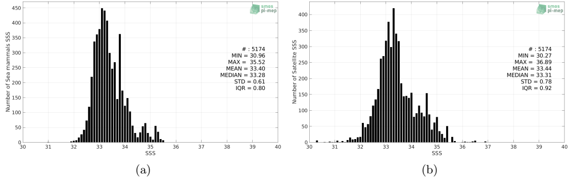
Figure 2: Histograms of SSS from Sea mammals (a) and SMOS SSS L3 v3 Monthly (ICDC) (b) considering all match-up pairs per bins of 0.1 over the Mid-Low Latitudes 45N-45S Pi-MEP region and for the full satellite product period.
