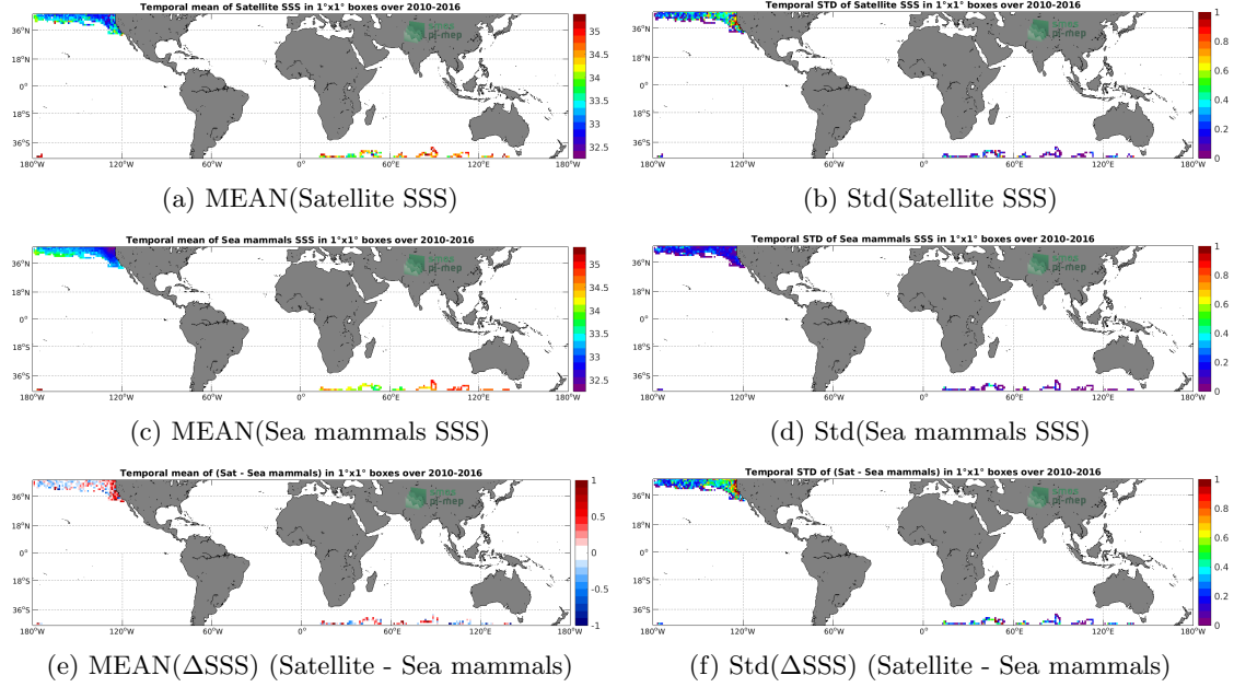
Figure 6: Temporal mean (left) and Std (right) of SSS from SMOS SSS L3 v3 Monthly (ICDC) (top), Sea mammals (middle), and of \Delta SSS (Satellite - Sea mammals). Only match-up pairs are used to generate these maps.
