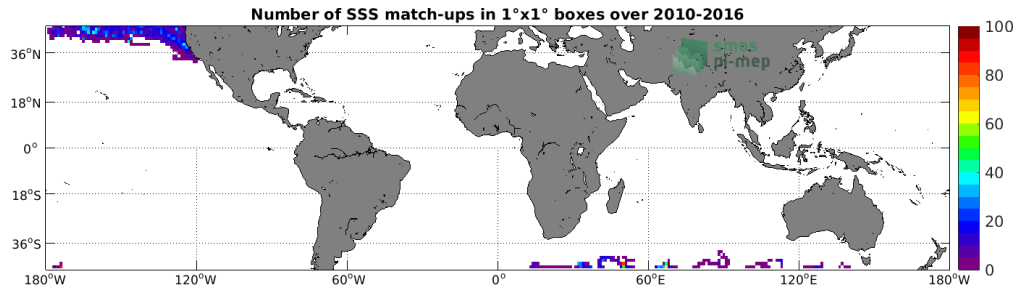
Figure 4: Number of SSS match-ups between Sea mammals SSS and the SMOS SSS L3 v3 Monthly (ICDC) SSS product for the Mid-Low Latitudes 45N-45S Pi-MEP region over 1°x1° boxes and for the full satellite product period.
