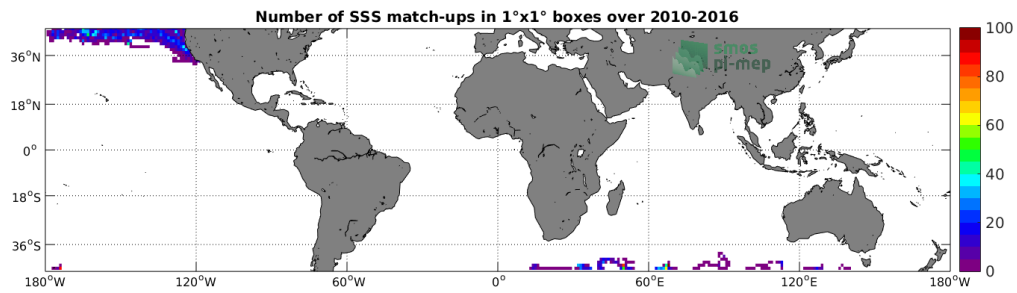
Figure 4: Number of SSS match-ups between Sea mammals SSS and the SMOS-L3-ICDC-V3-MONTHLY-0.5DEG SSS product for the Mid-Low Latitudes 45N-45S Pi-MEP region over 1°x1° boxes and for the full satellite product period.
